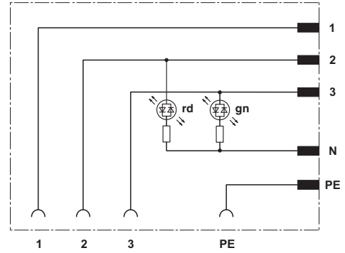
Circuit diagram
