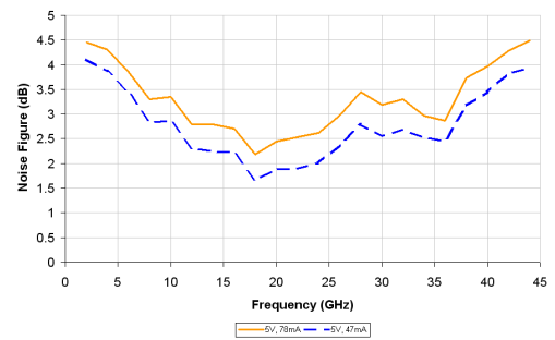
Noise Figure
