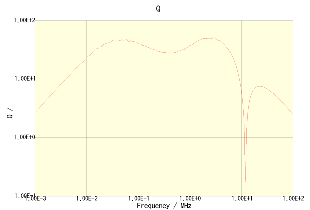
CLF10040T-470M-CA
