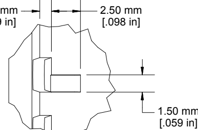
DETAIL C SCALE 3 : 1 Interior Features
