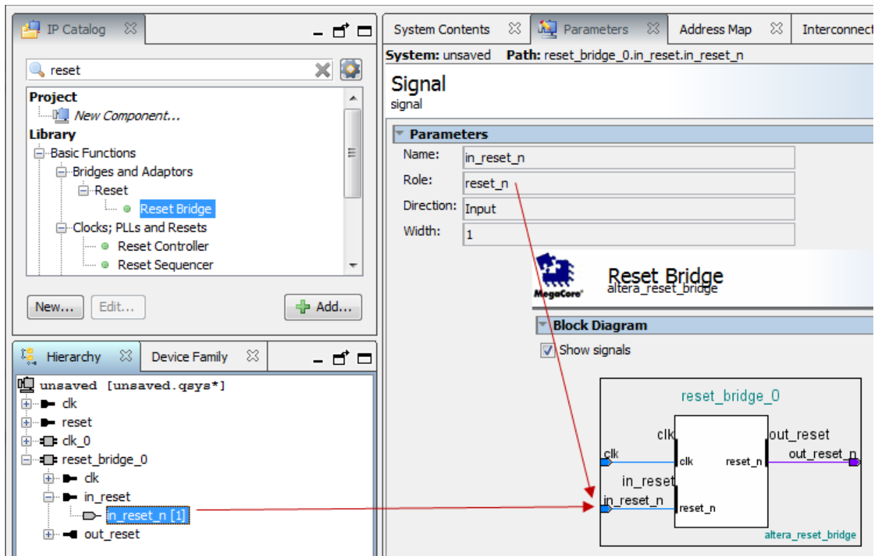
Figure 8-29: Reset Signal Active-Low
