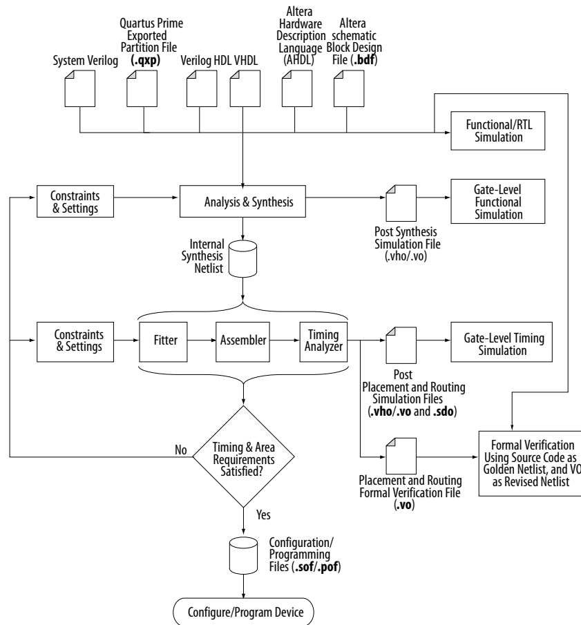
Figure 16-1: Basic Design Flow Using Quartus Prime Integrated Synthesis
