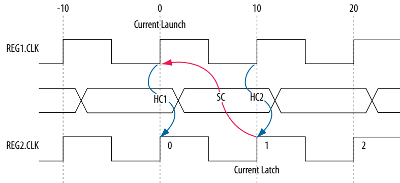
Figure 7-18: Default Timing Diagram
