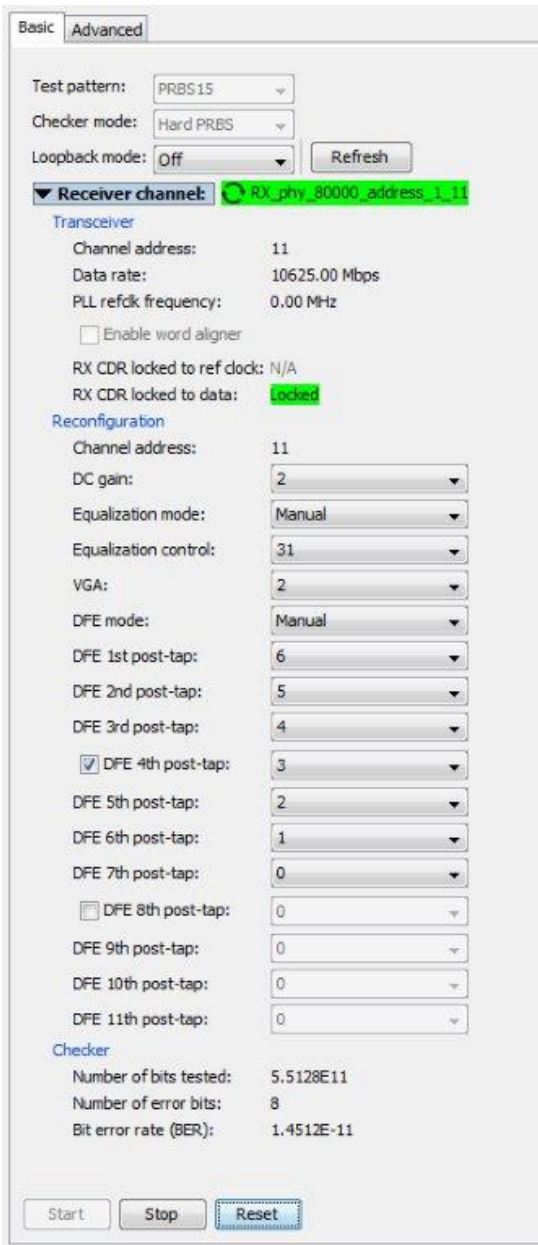
Figure 11-20: Controlling Receiver Channel
