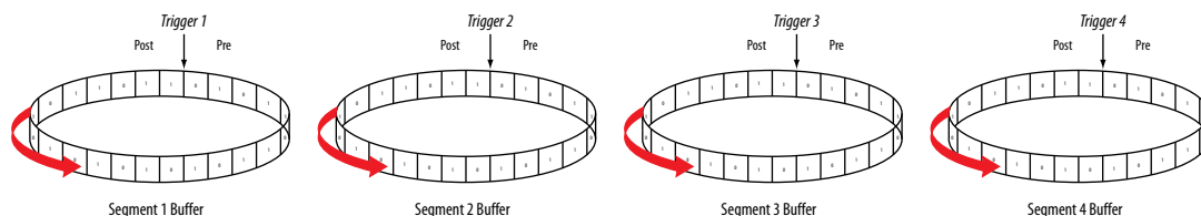
Figure 13-50: Segmented Acquisition Buffer
