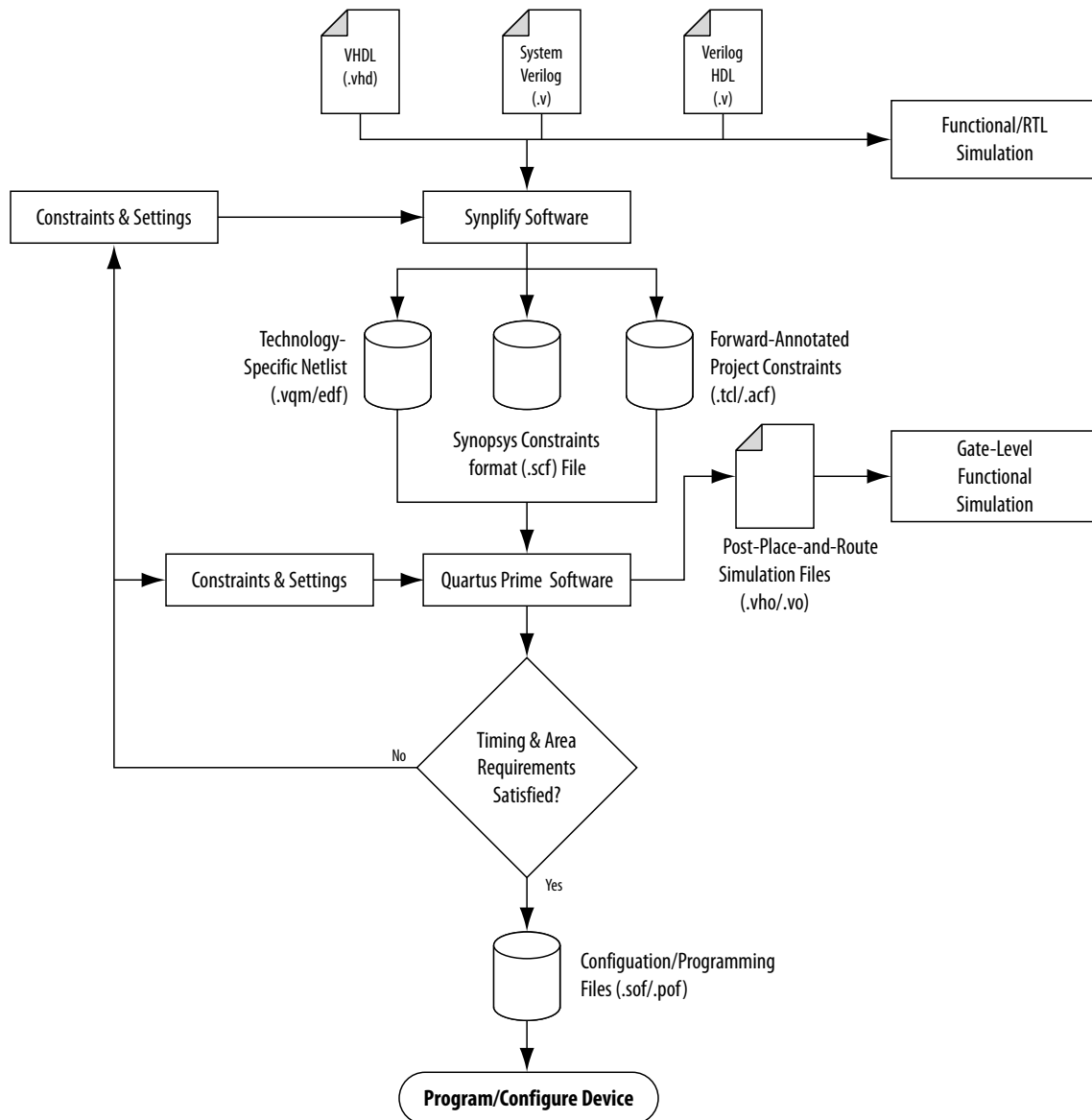
Figure 18-1: Recommended Design Flow
