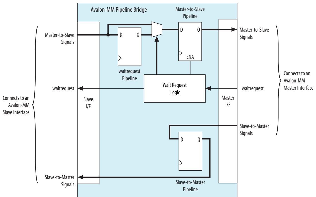
Figure 8-9: Avalon-MM Pipeline Bridge
