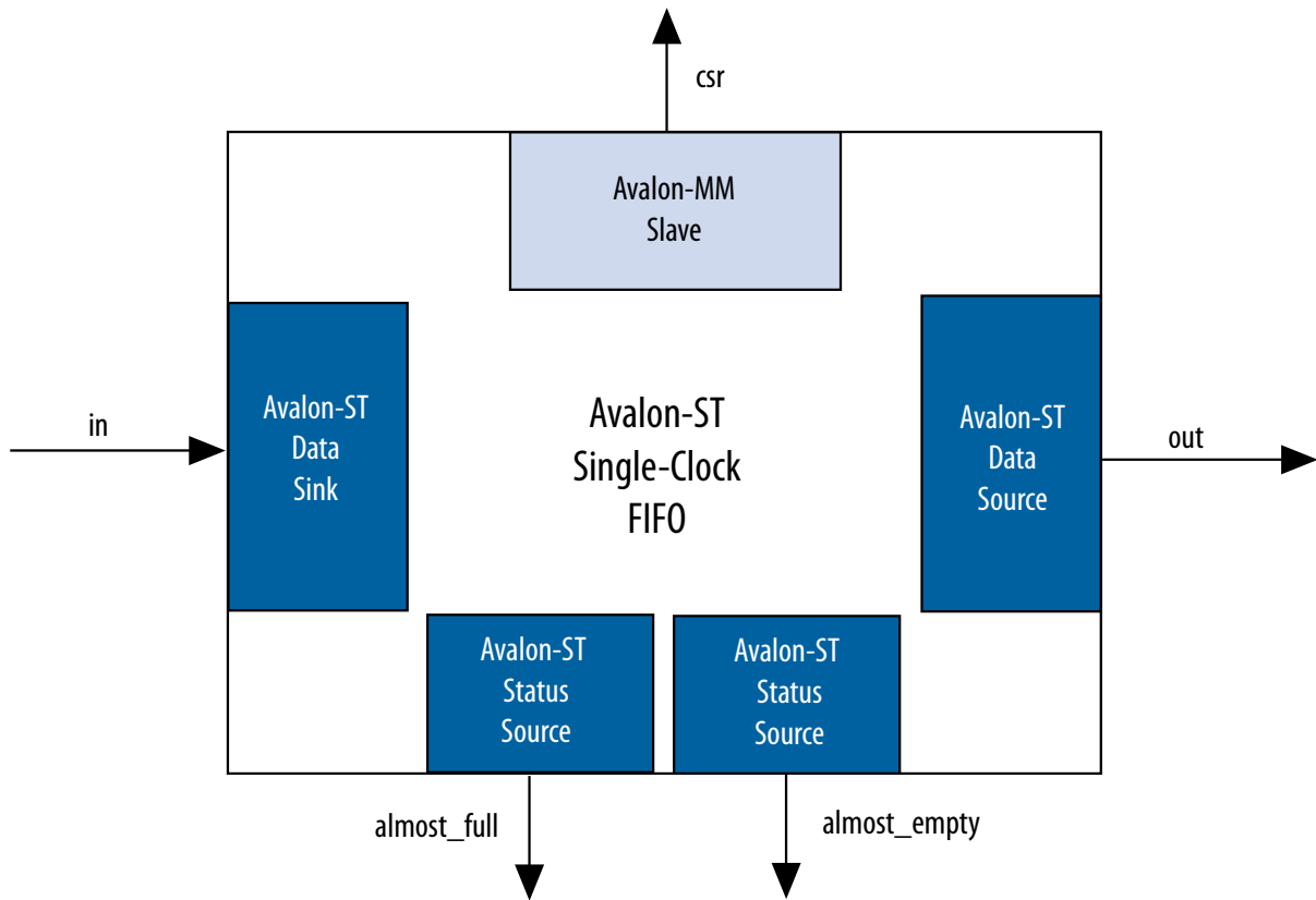
Figure 10-37: Avalon-ST Single Clock FIFO Core
