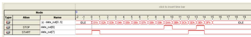
Figure 13-18: Data Acquisition of a Recurring Data Pattern in Continuous Mode (Start/Stop)
