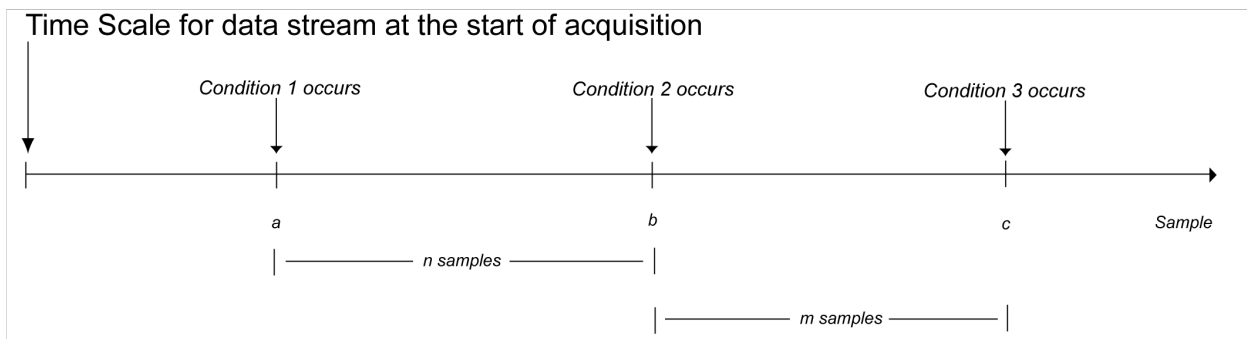
Figure 13-38: Capture Scenario for Storage Qualification with the State-Based Trigger Flow
