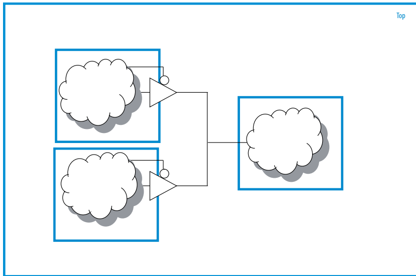
Figure 14-15: Unsupported Internal Tri-State Signals
