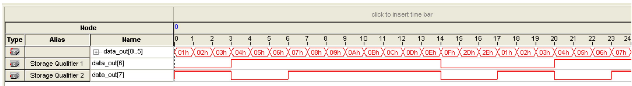
Figure 13-15: Data Acquisition of a Recurring Data Pattern in Continuous Capture Mode (Conditional)
