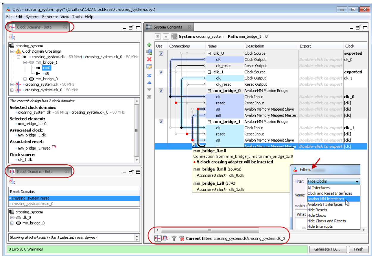
Figure 5-25: Qsys Clock and Reset Domains
