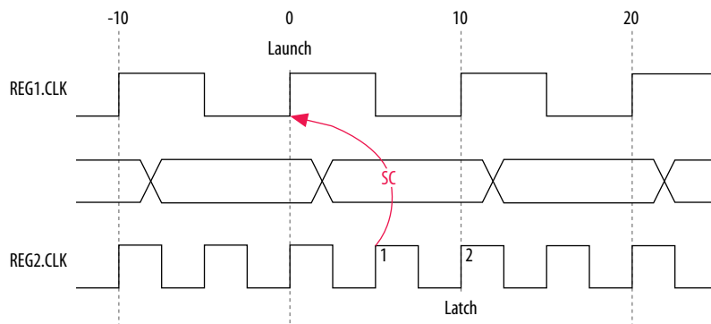
Figure 7-43: Setup Timing Diagram
