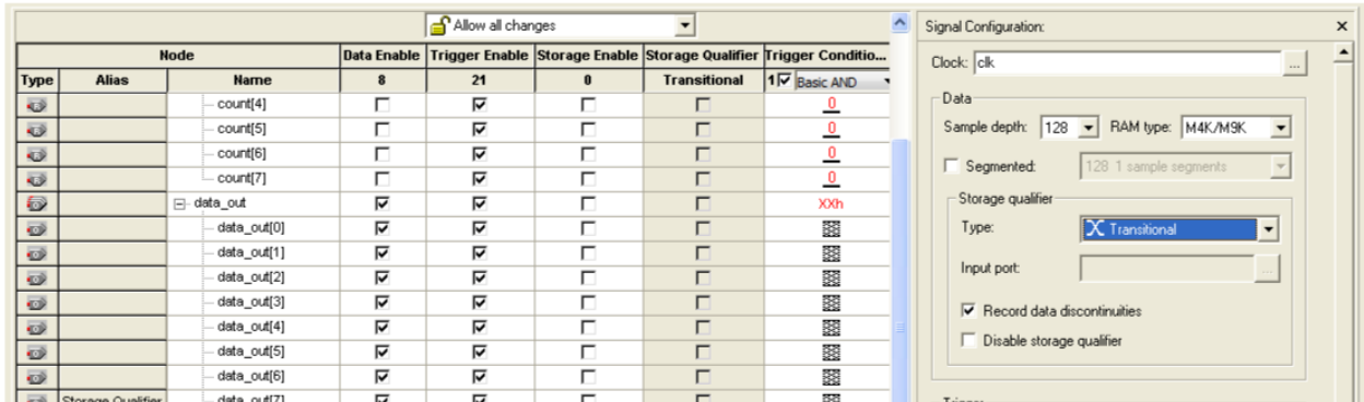
Figure 13-12: Data Acquisition of a Recurring Data Pattern in Continuous Capture Mode (Transitional Mode)
