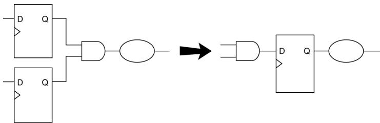
Figure 16-2: Combining Registers with Register Retiming
