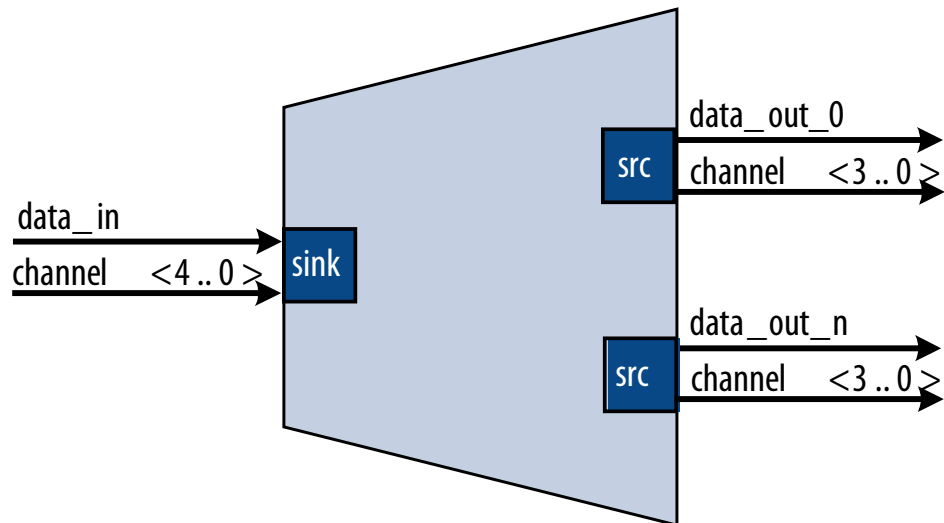
Figure 10-36: Select Bits for the Demultiplexer
