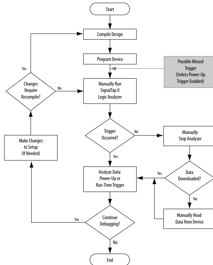
Figure 13-48: Power-Up and Runtime Trigger Events Flowchart
