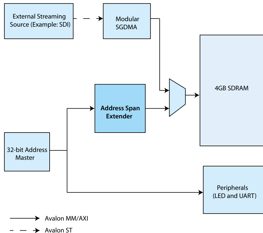
Figure 10-17: Block Diagram with Address Span Extender
