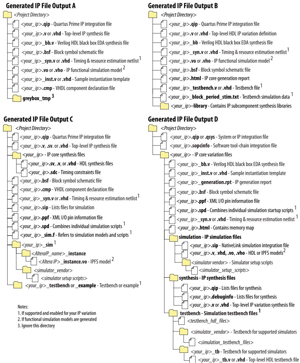
Figure 5-34: IP Core Generated Files (Legacy Parameter Editors)
