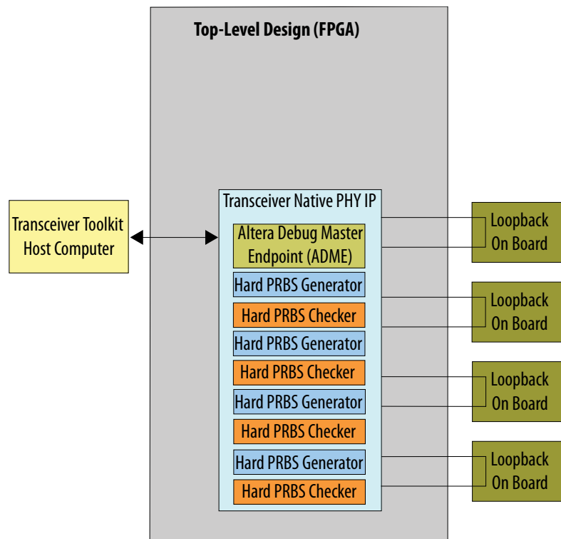
Figure 11-16: Four Channel Loopback Mode for Arria 10 / Generation 10 / 20nm
