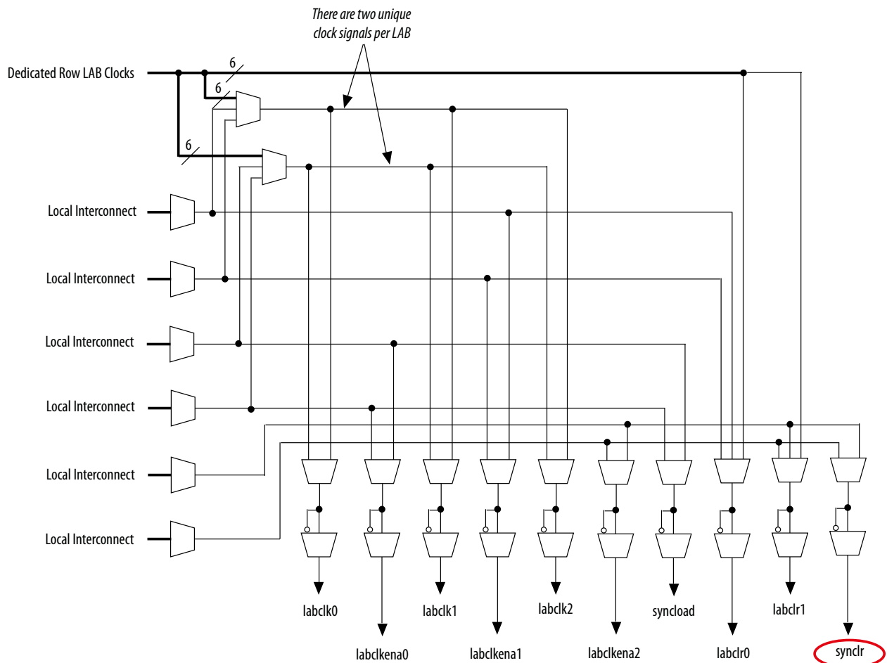
Figure 11-15: LAB-Wide Control Signals
