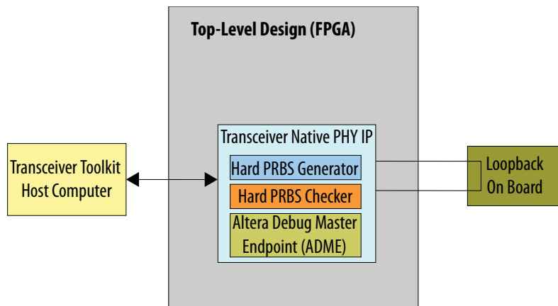
Figure 11-14: One Channel Loopback Mode for Arria 10 / 20nm
