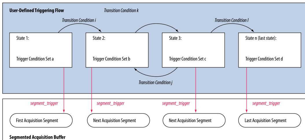
Figure 13-37: State-Based Triggering Flow
