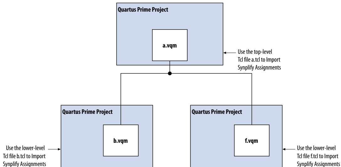
Figure 18-8: Design Flow Using Multiple Synplify Projects and Multiple Quartus Prime Projects
