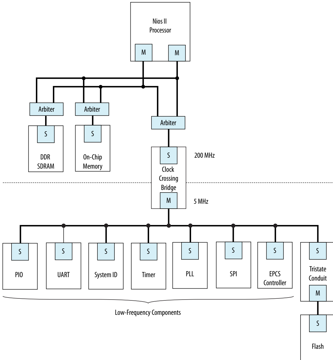
Figure 8-25: Reducing Power Utilization Using a Bridge to Separate Clock Domains
