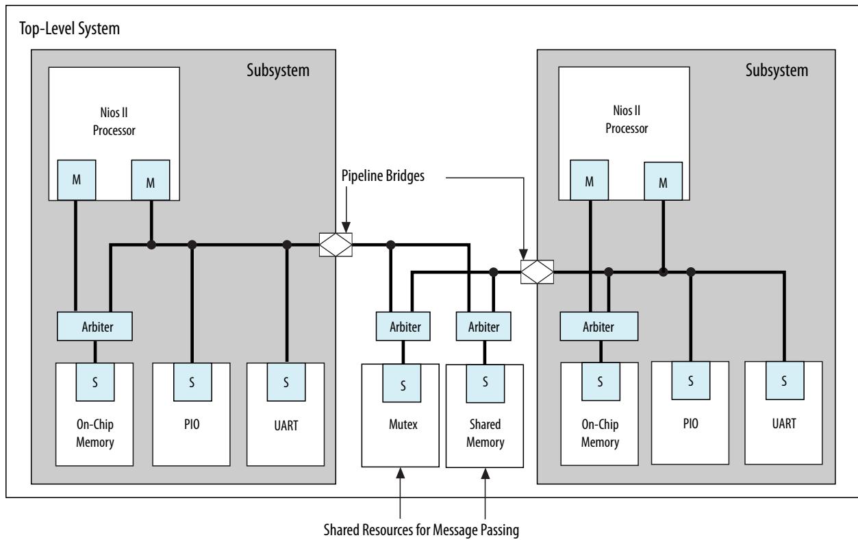
Figure 8-3: Passing Messages Between Subsystems
