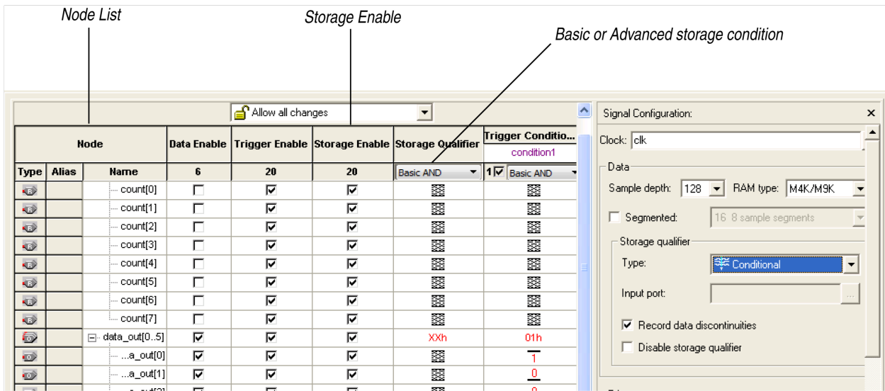
Figure 13-14: Conditional Storage Qualifier Setup
