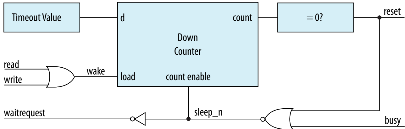
Figure 8-27: Hardware-Controlled Sleep Components
