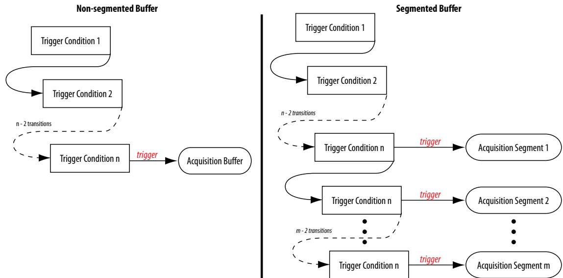
Figure 13-36: Sequential Triggering Flow
