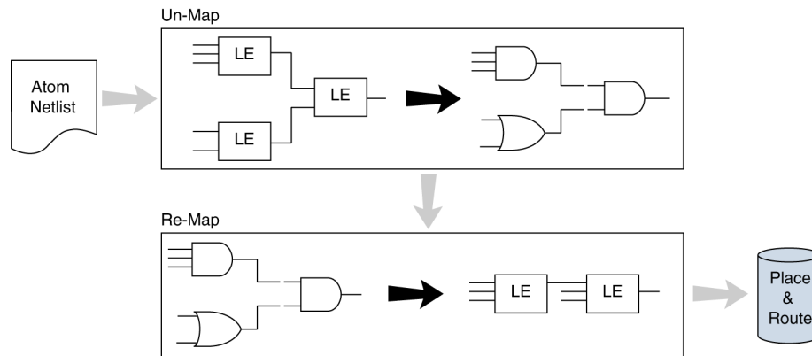
Figure 16-3: Quartus Prime Flow for WYSIWYG Primitive Resynthesis
