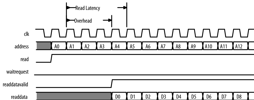
Figure 8-13: High Efficiency Read Transfer
