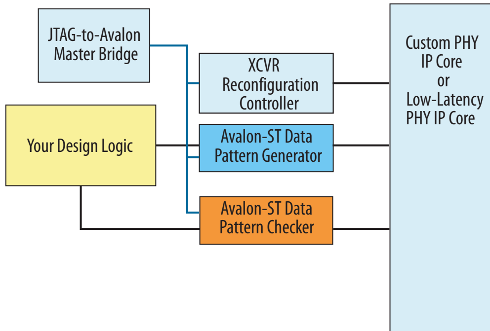
Figure 11-8: PRBS Signal Eye Test Configuration (Stratix V)
