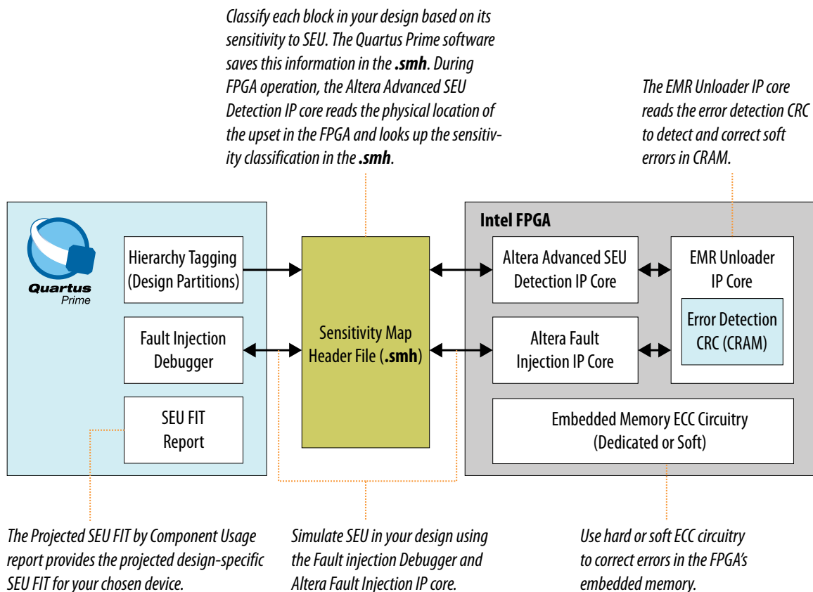
Figure 15-1: Tools, IP, and Circuitry for Detecting and Correcting SEU
