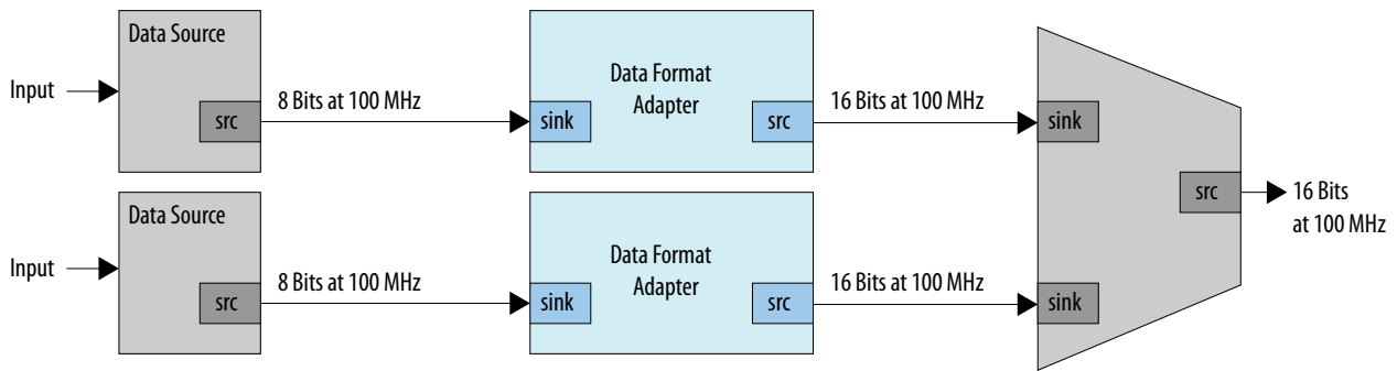
Figure 8-35: Datapath to Double Data Width and Maintain Original Frequency
