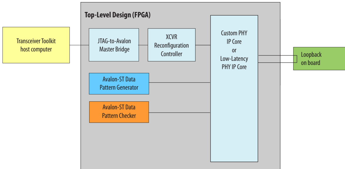
Figure 11-13: One Channel Loopback Mode for Stratix V / 28nm
