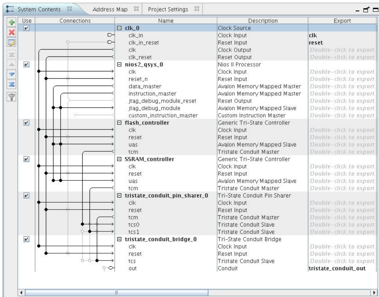
Figure 10-24: Tri-State Conduit System in Qsys
