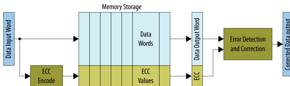
Figure 15-2: Memory Storage and ECC
