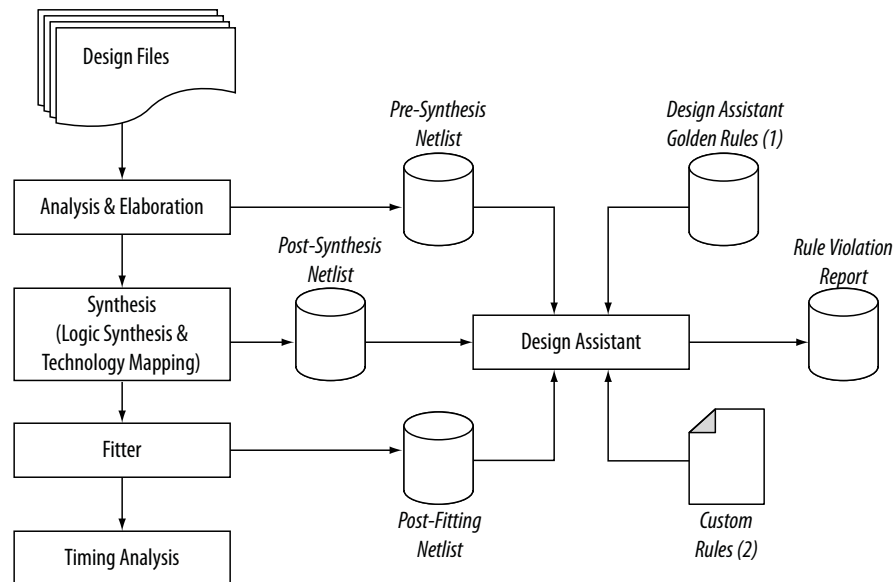
Figure 11-9: Quartus Prime Design Flow with the Design Assistant
