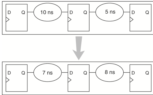
Figure 16-1: Reducing Critical Delay by Moving the Register Relative to Combinational Logic
