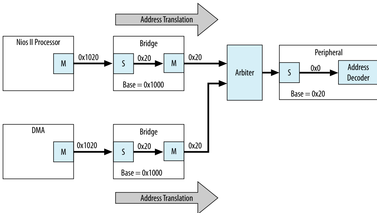
Figure 8-20: Address Translation Corrected With Bridge
