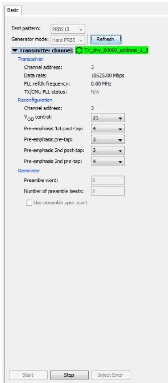
Figure 11-19: Controlling Transmitter Channel
