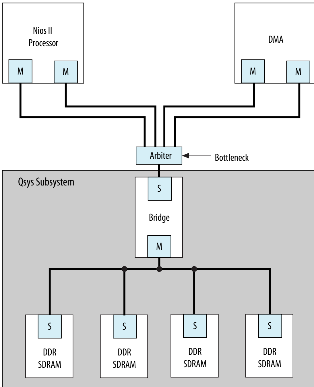
Figure 8-16: Inappropriate Use of a Bridge in a Hierarchical System
