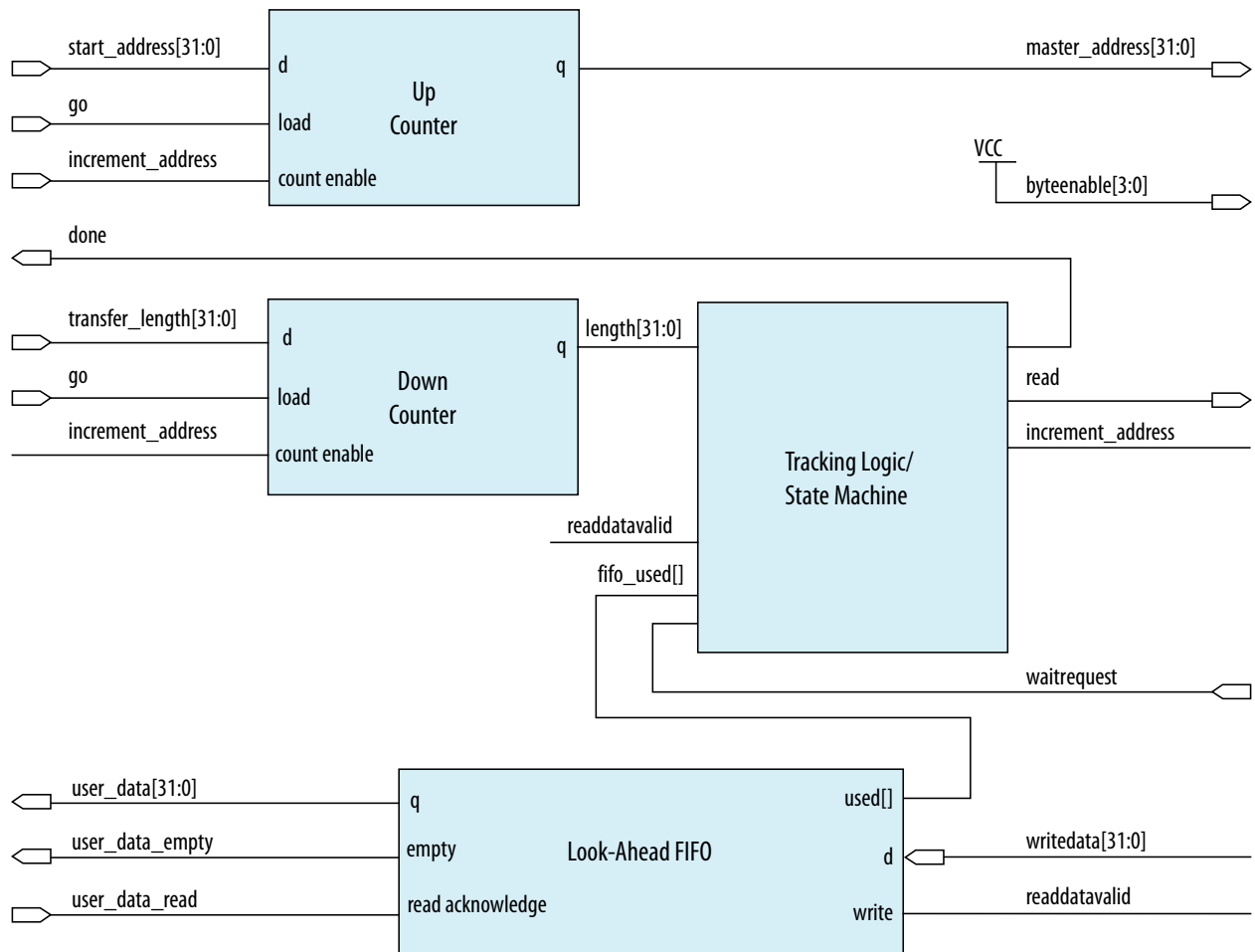
Figure 8-33: Pipelined Read Master
