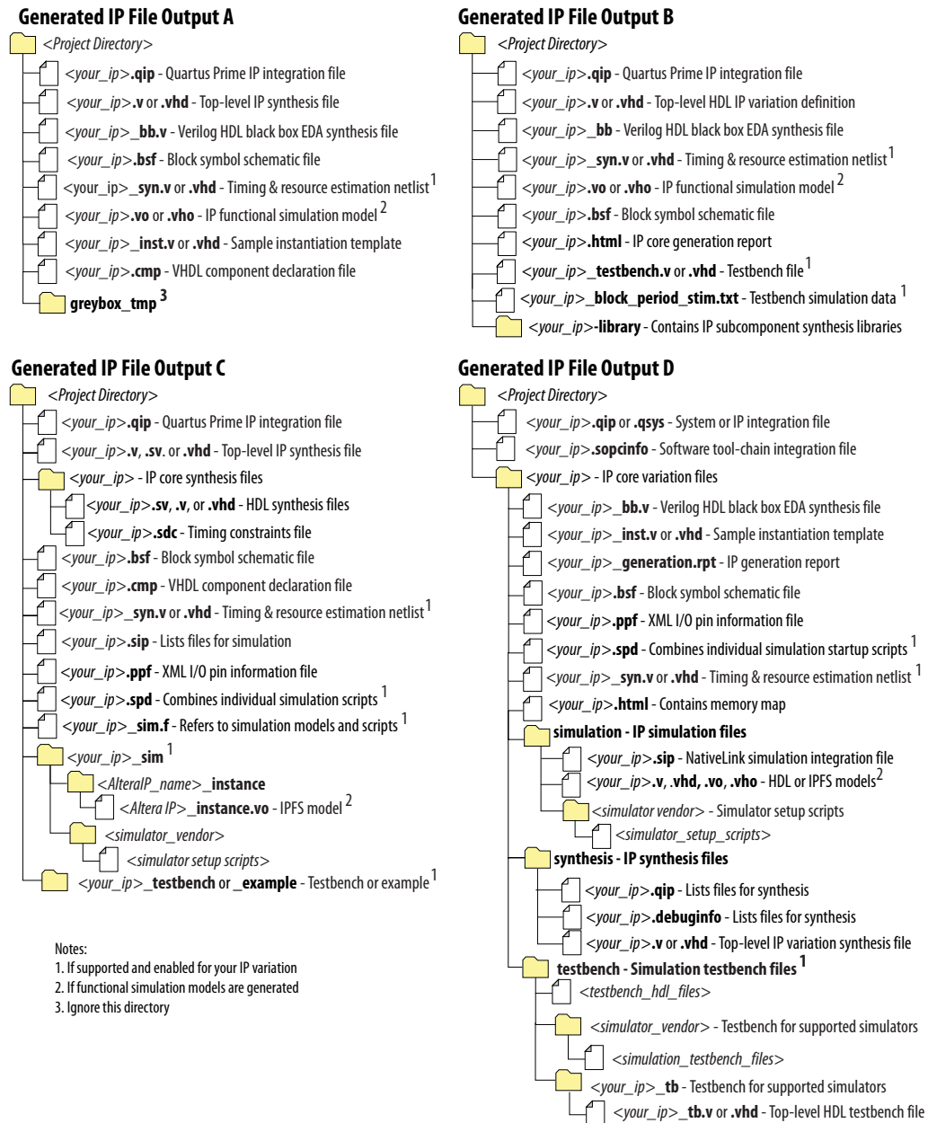
Figure 1-16: IP Core Generated Files (Legacy Parameter Editors)
