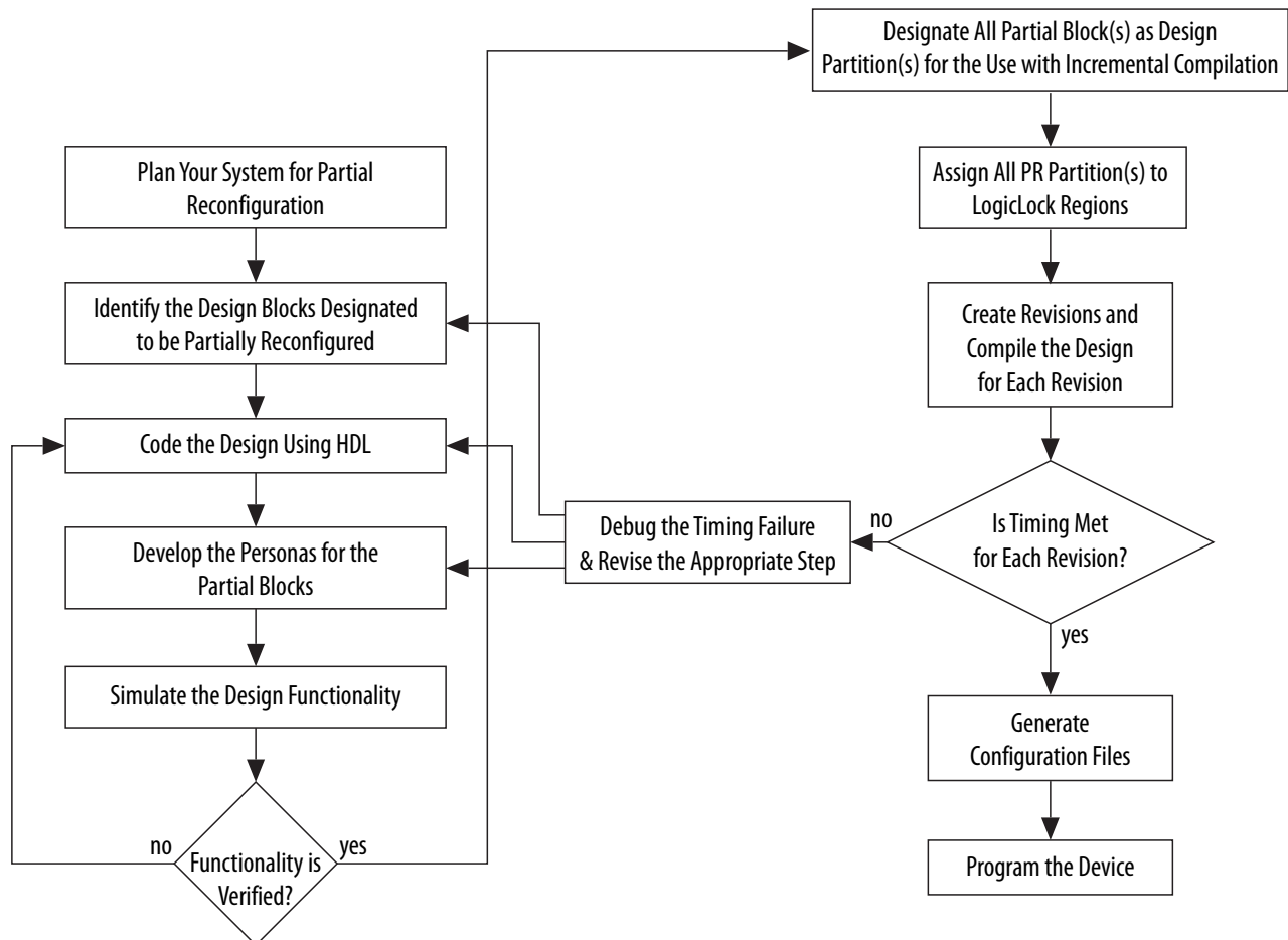
Figure 4-7: Partial Reconfiguration Design Flow
