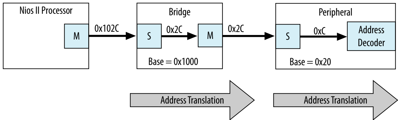
Figure 8-18: Bridge Address Translation
