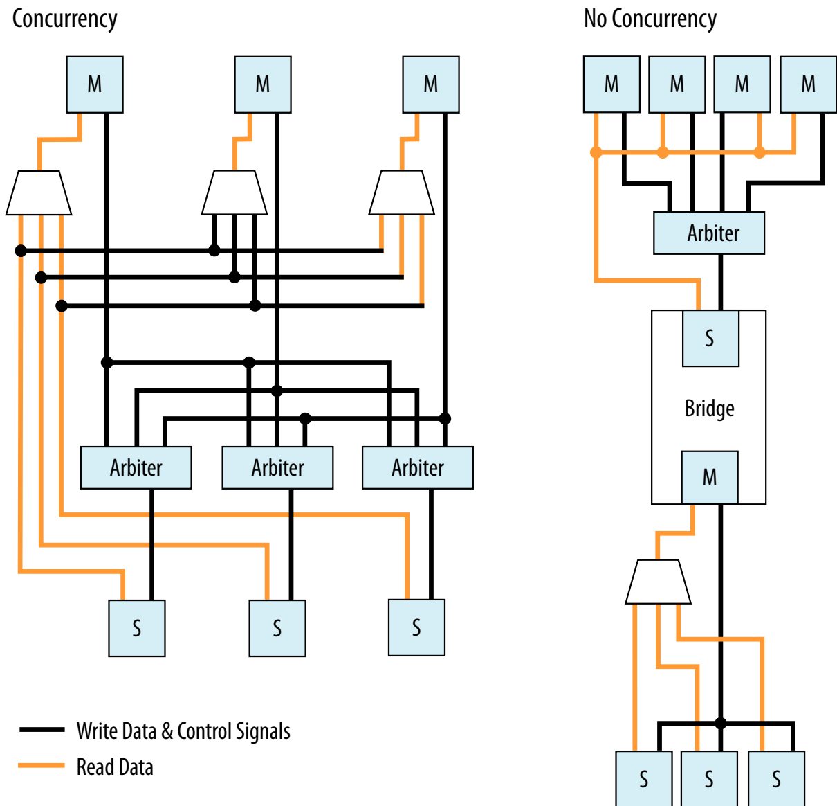
Figure 8-11: Differences Between Systems With and Without a Pipeline Bridge
