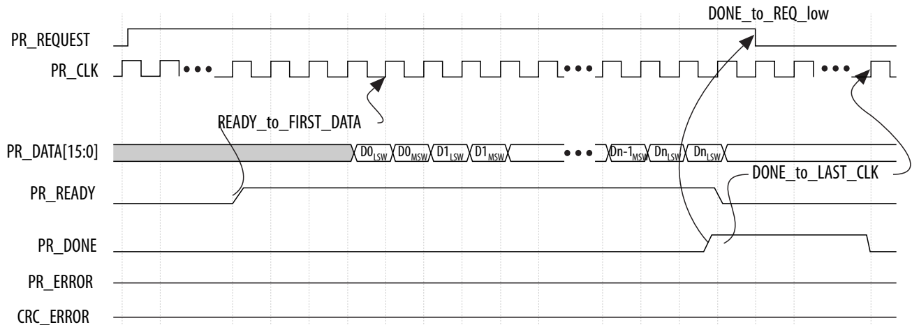
Figure 4-13: Partial Reconfiguration Timing Diagram
