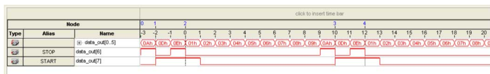
Figure 13-19: Data Acquisition of a Recurring Data Pattern with Start/Stop Storage Qualifier Enabled
