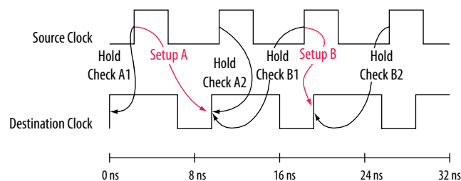
Figure 6-11: Setup and Hold Check Relationships
