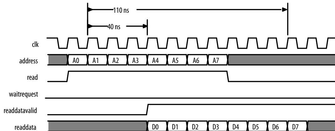
Figure 8-14: Performance of a Nios II Processor and Memory Operating at 100 MHz
