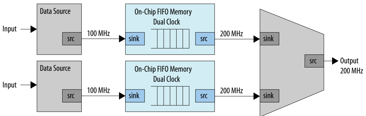
Figure 8-36: Datapath to Boost the Clock Frequency
