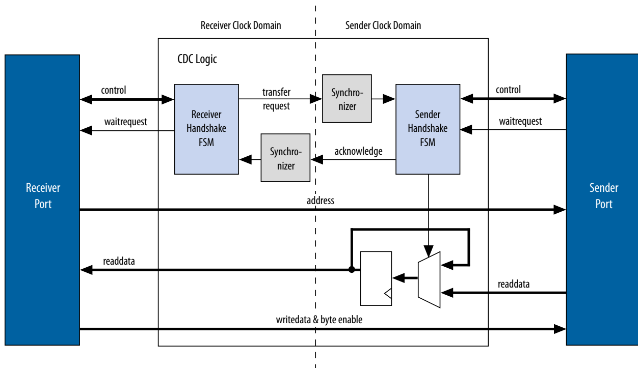
Figure 8-24: Clock Crossing Adapter
