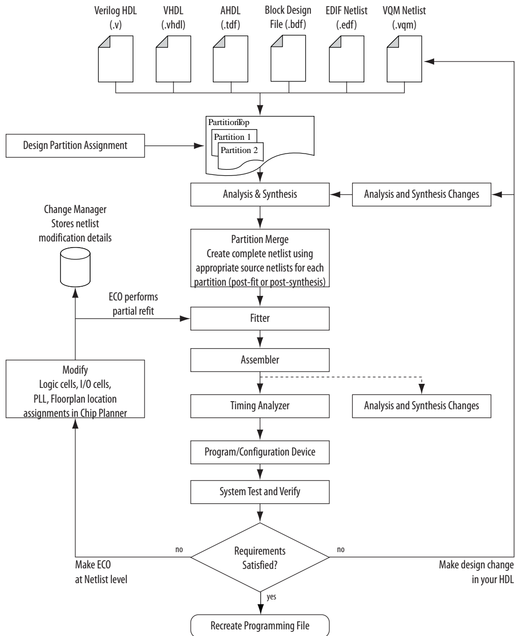
Figure 17-1: Design Flow to Support ECOs
