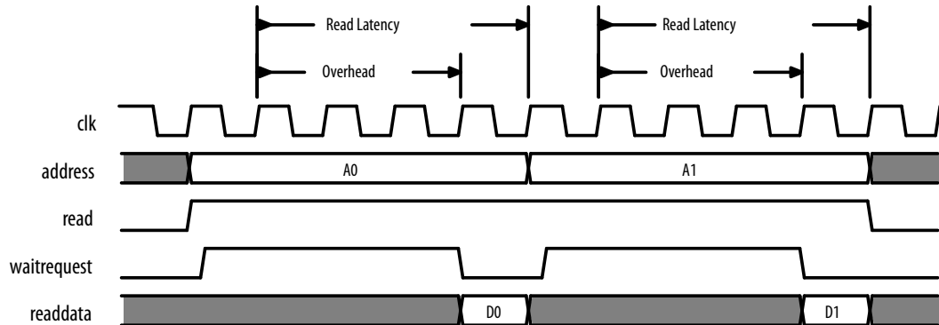
Figure 8-12: Low-Efficiency Read Transfer
