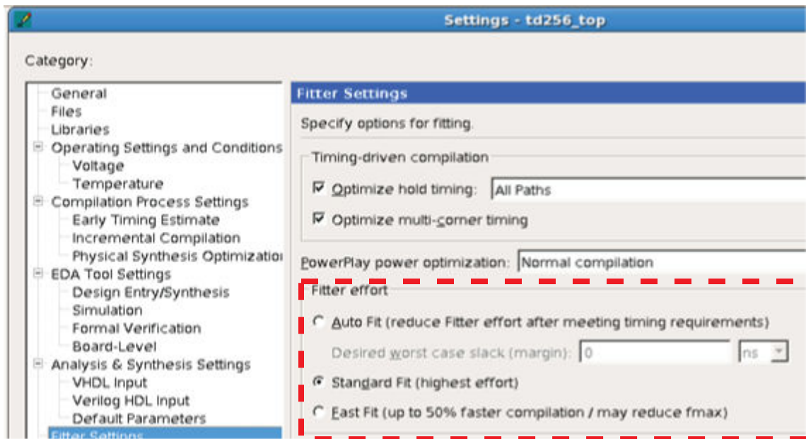
Figure 12-19: Fitter Effort
