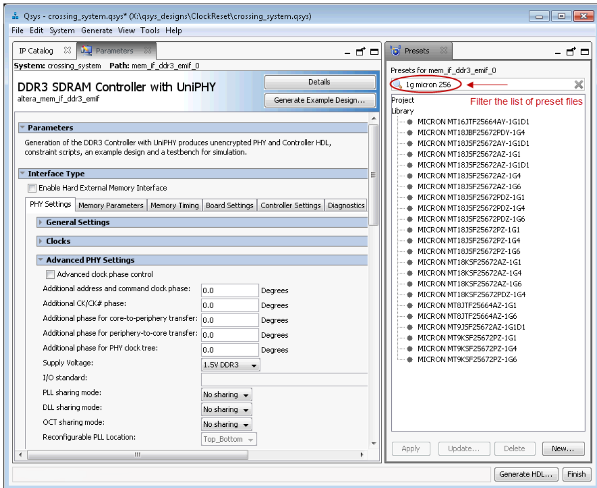
Figure 5-13: Specifying Presets
