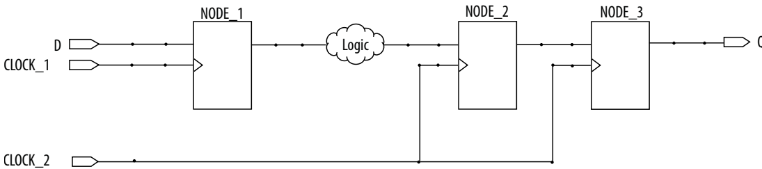
Figure 11-12: Undesired Condition 3
