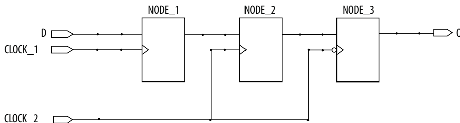
Figure 11-13: Undesired Condition 4
