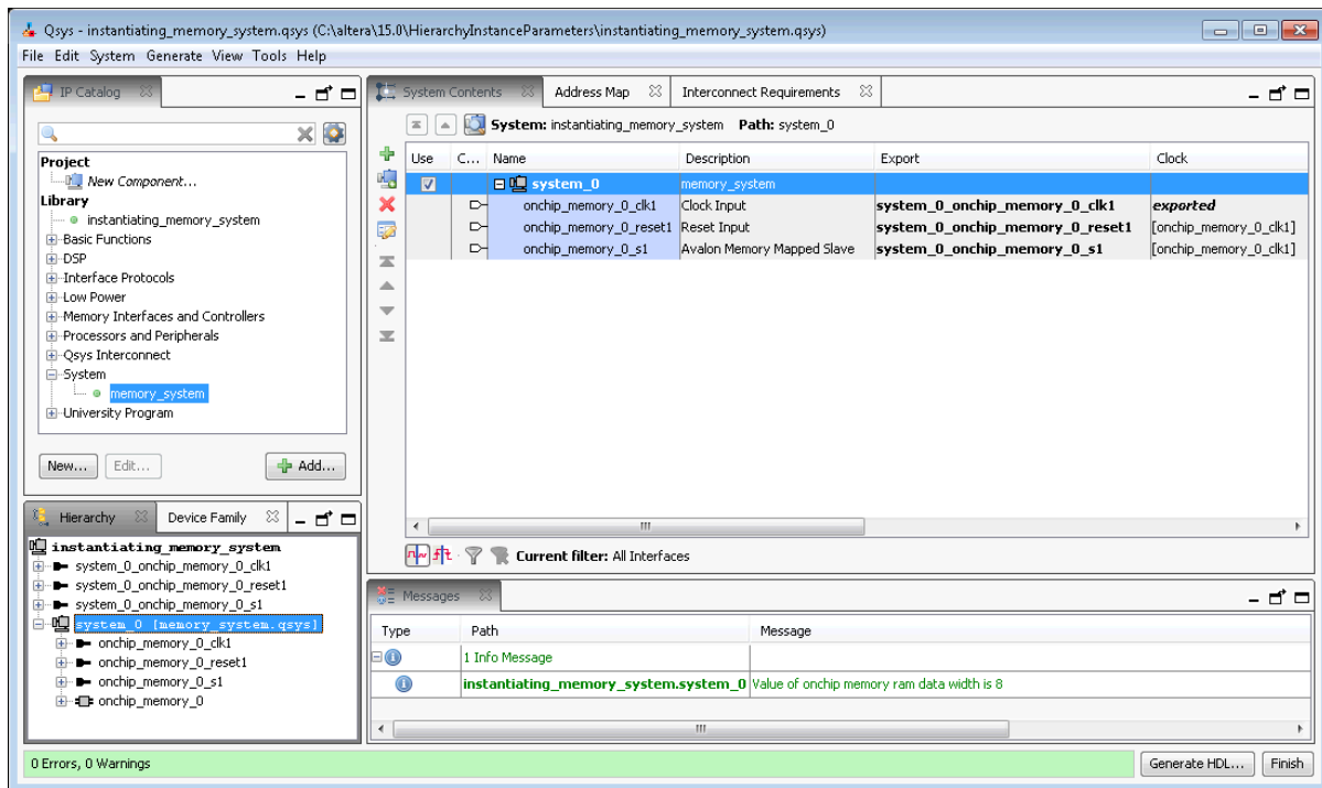
Figure 5-22: Instantiating Memory System (instantiating_memory_system.qsys)
