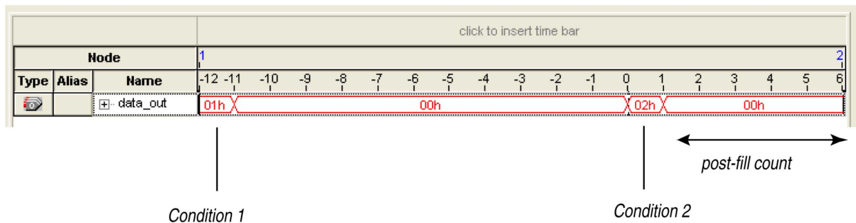
Figure 13-39: Storage Qualification with Post-Fill Count Value Less than m (Acquisition Successfully Completes)
