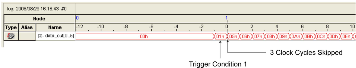
Figure 13-43: Capture of Data Transaction with Trigger Flow Description Applied
