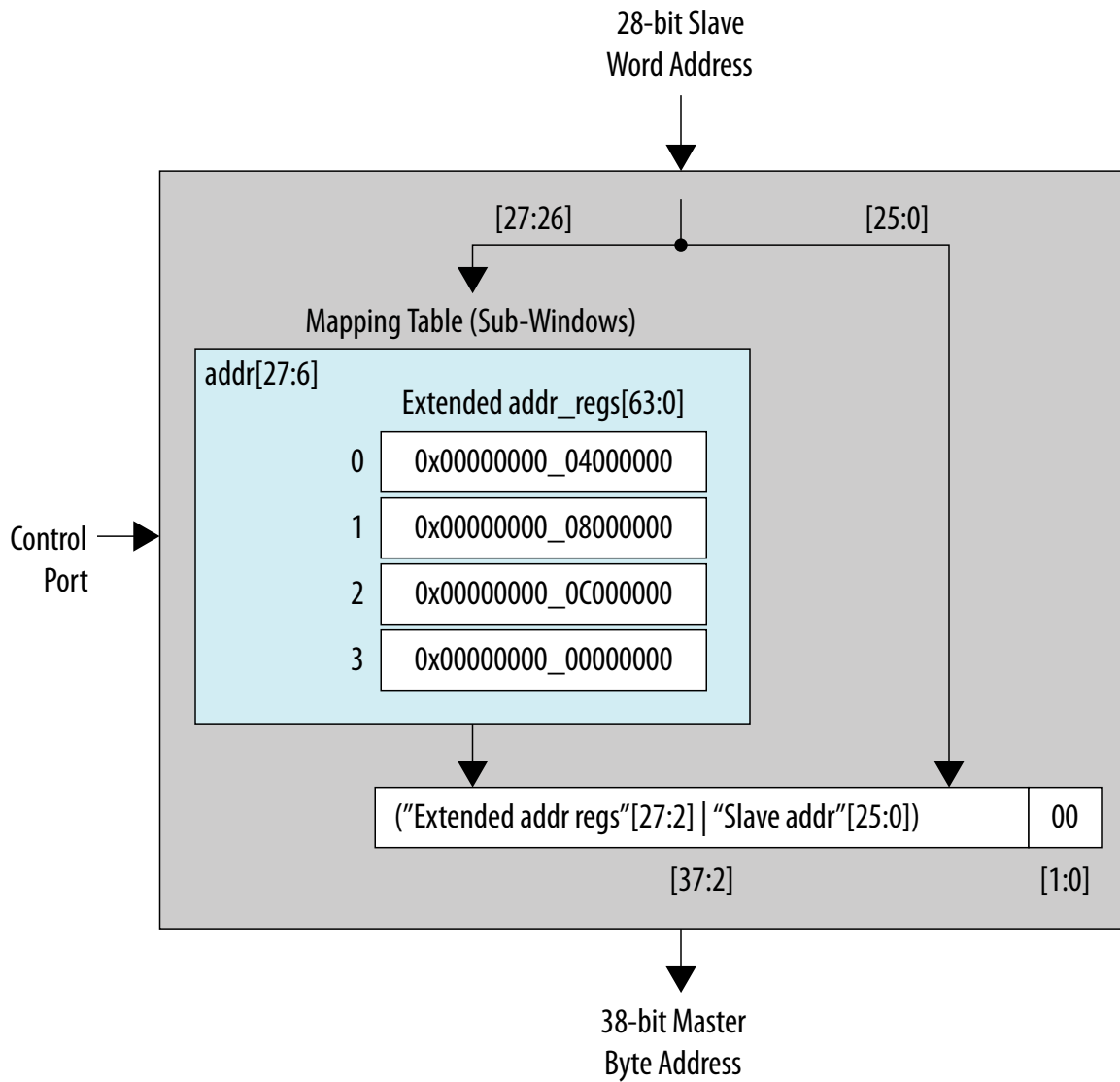
Figure 10-16: Address Span Extender
