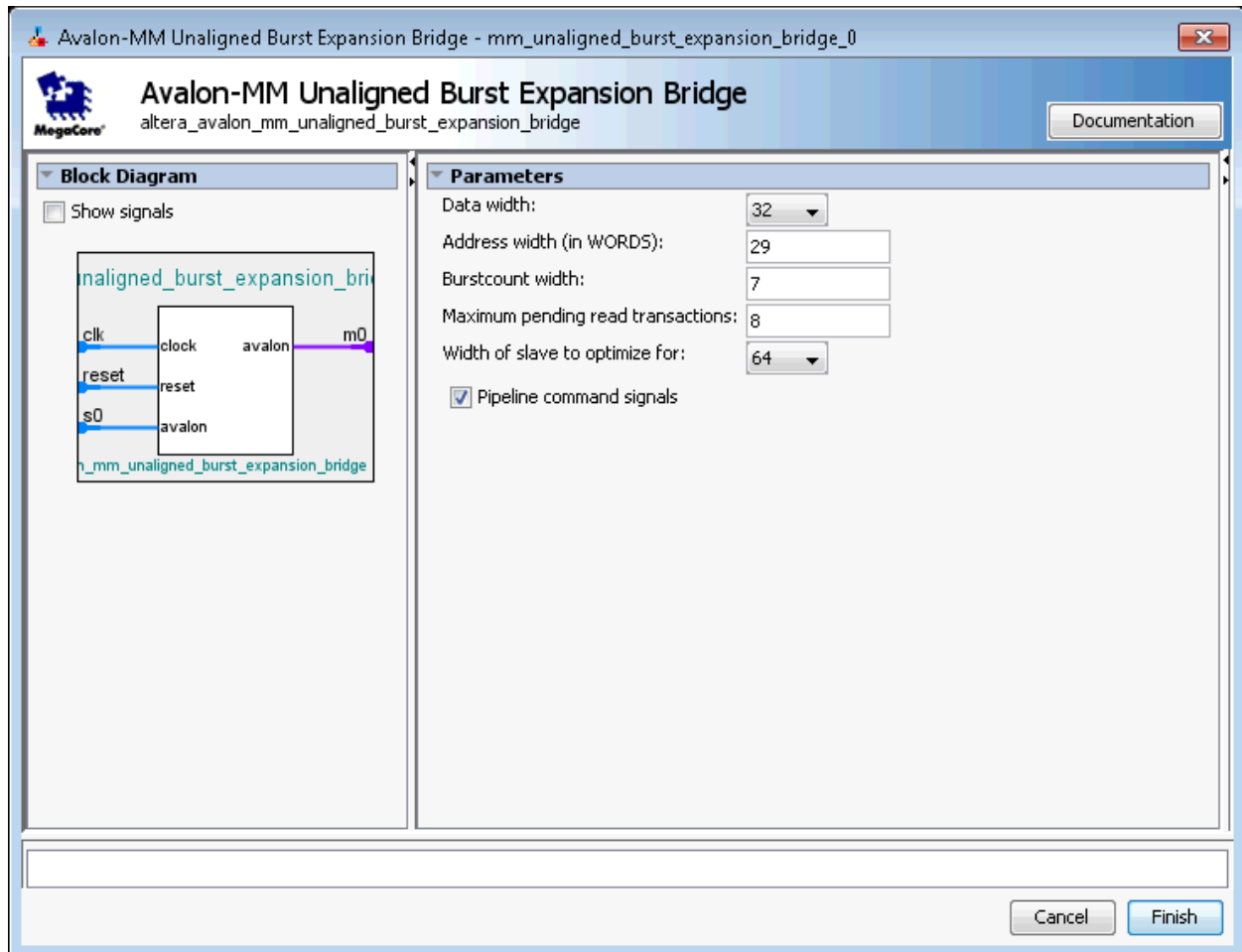
Figure 10-6: Avalon-MM Unaligned Burst Expansion Bridge Parameter Editor
