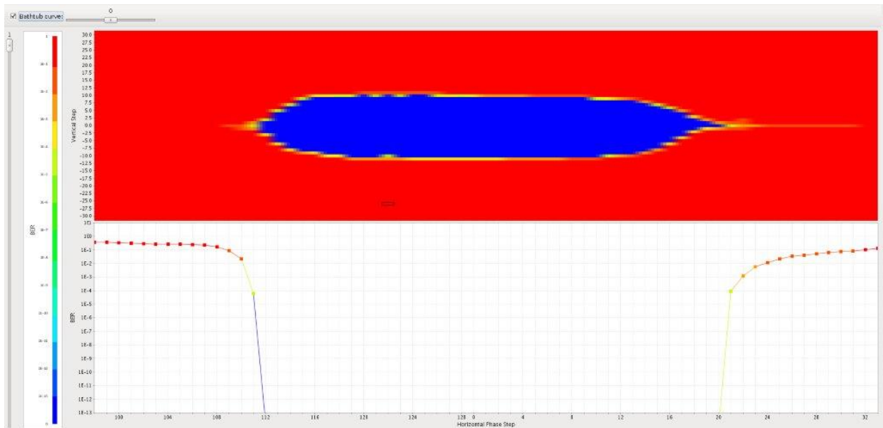
Figure 11-18: Heat Map Display and Bathtub Curve Through Eye
