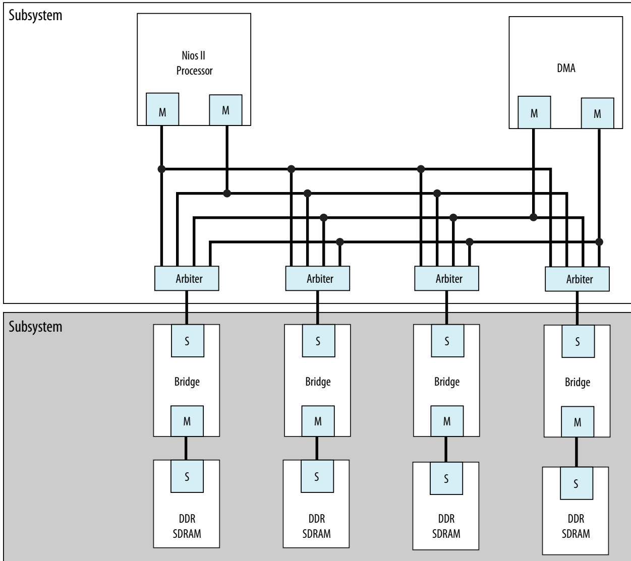
Figure 8-17: Efficient Memory Pipelining Without a Bottleneck in a Hierarchical System
