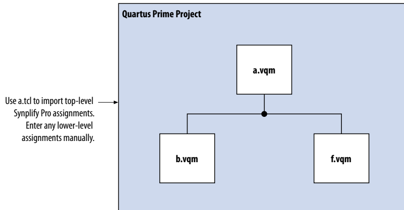
Figure 18-7: Design Flow Using Multiple .vqm Files with One Quartus Prime Project
