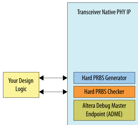
Figure 11-5: BER, PRBS, and Link Optimization Test Configuration (Arria 10)
