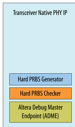
Figure 11-6: System Configuration: PMA Analog Setting Control (Arria 10)
