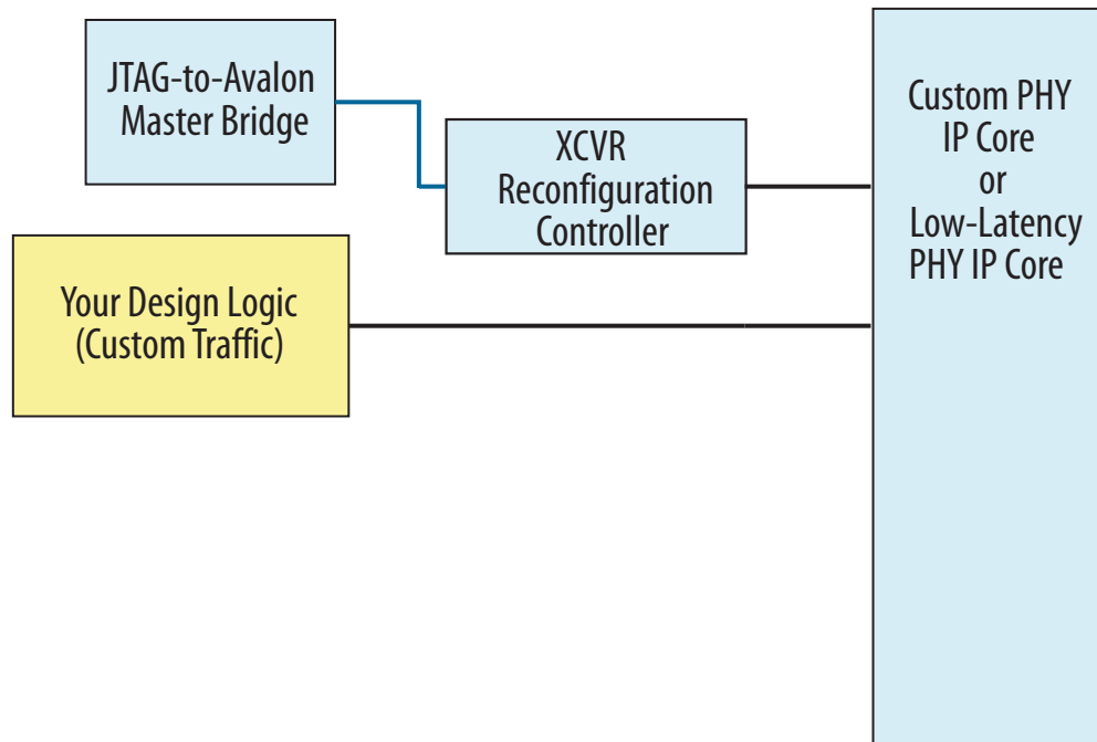
Figure 11-9: System Configuration: Custom Traffic Signal Eye Tests (Stratix V)
