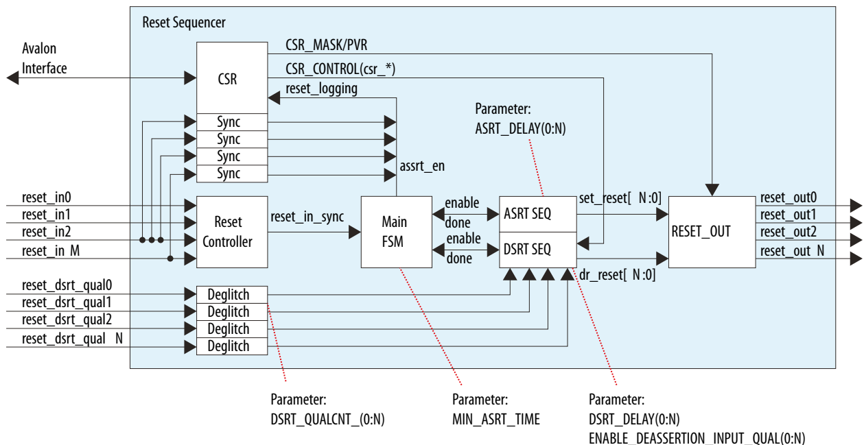
Figure 7-29: Elements and Flow of a Reset Sequencer
