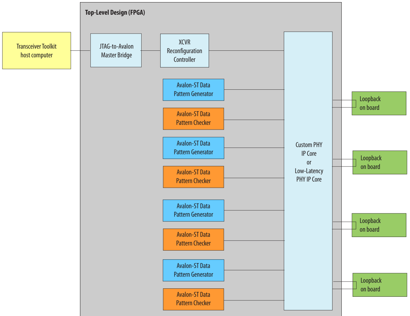
Figure 11-15: Four Channel Loopback Mode for Stratix V / 28nm
