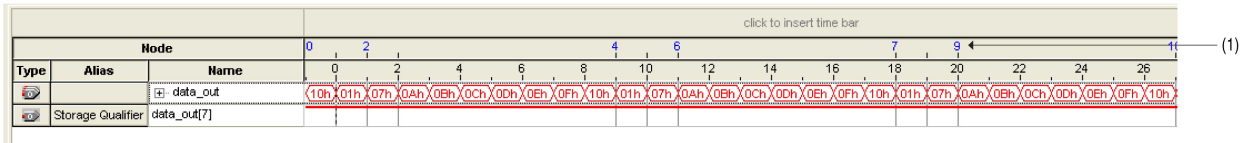
Figure 13-10: Data Acquisition of a Recurring Data Pattern Using an Input Signal as a Storage Qualifier
