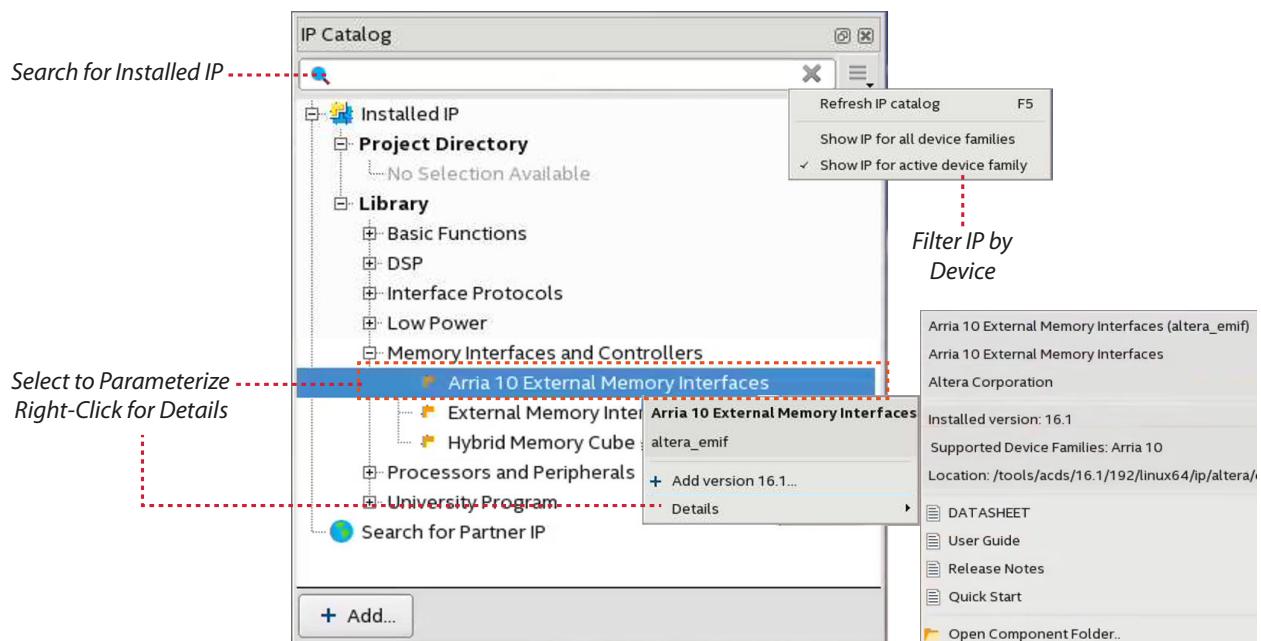
Figure 1-11: IP Catalog
