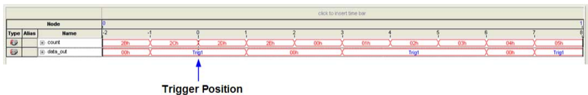
Figure 13-53: SignalTap II Logic Analyzer Conditional Data Capture
