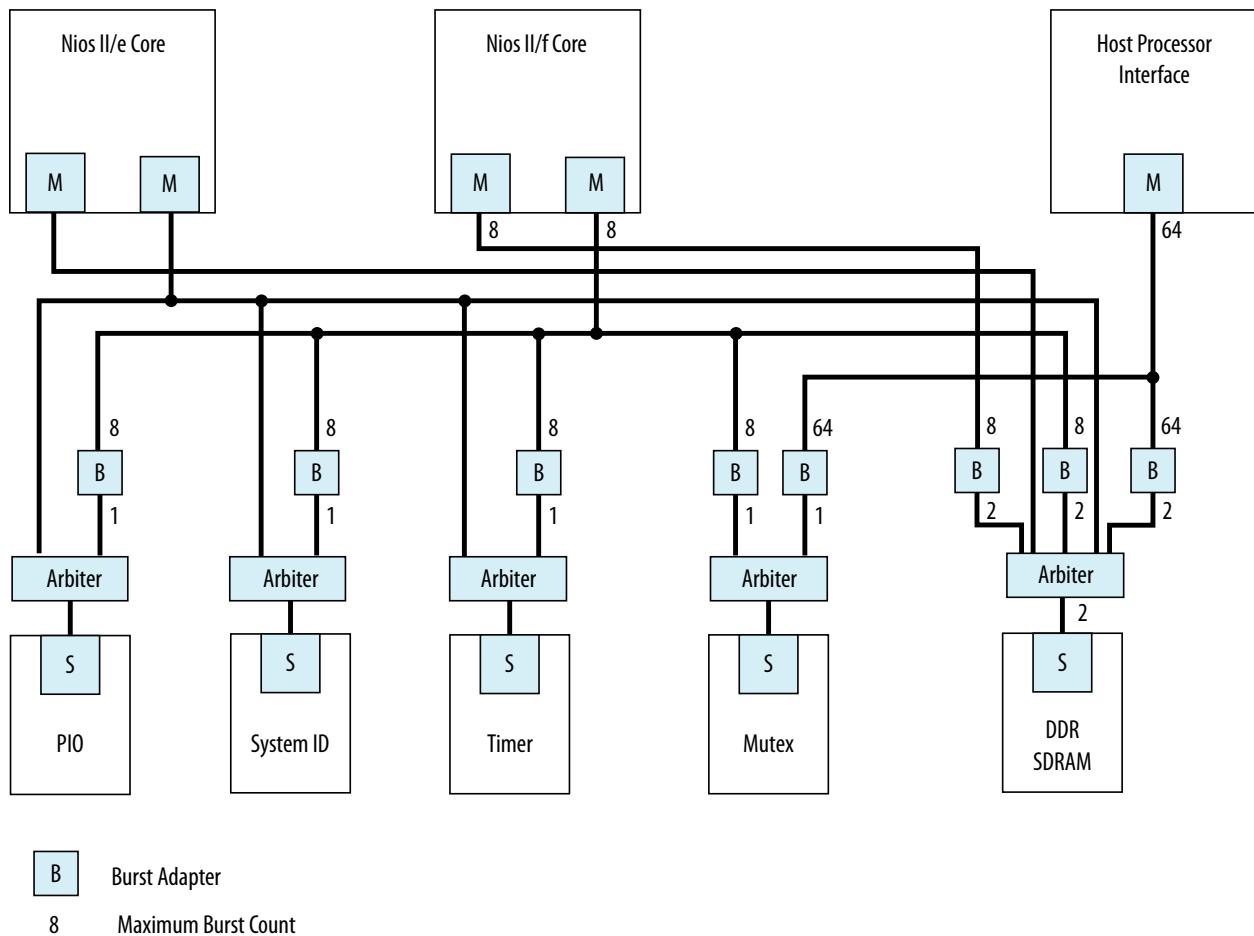
Figure 8-22: Mixed Bursting System
