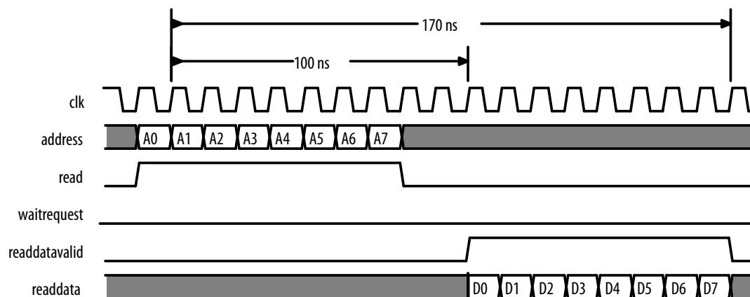
Figure 8-15: Performance of a Nios II Processor and Eight Reads with Ten Cycles Latency
