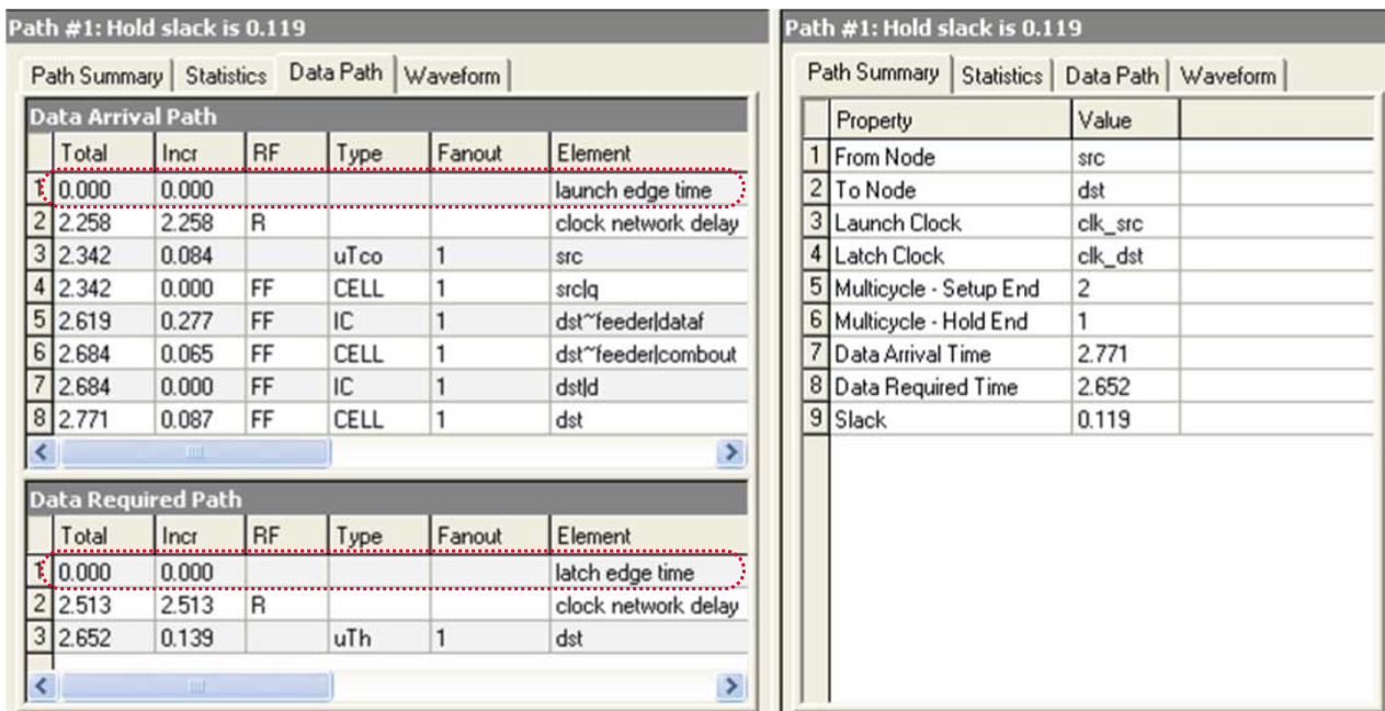
Figure 7-34: Hold Report
