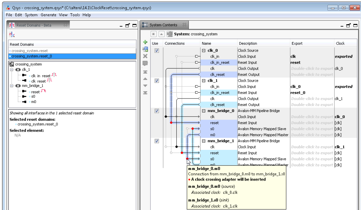
Figure 5-30: Reset Domains
