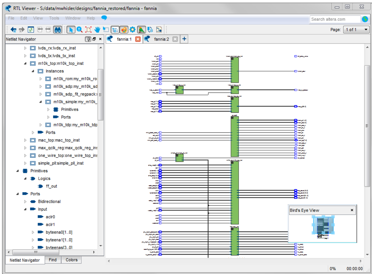
Figure 17-2: RTL Viewer
