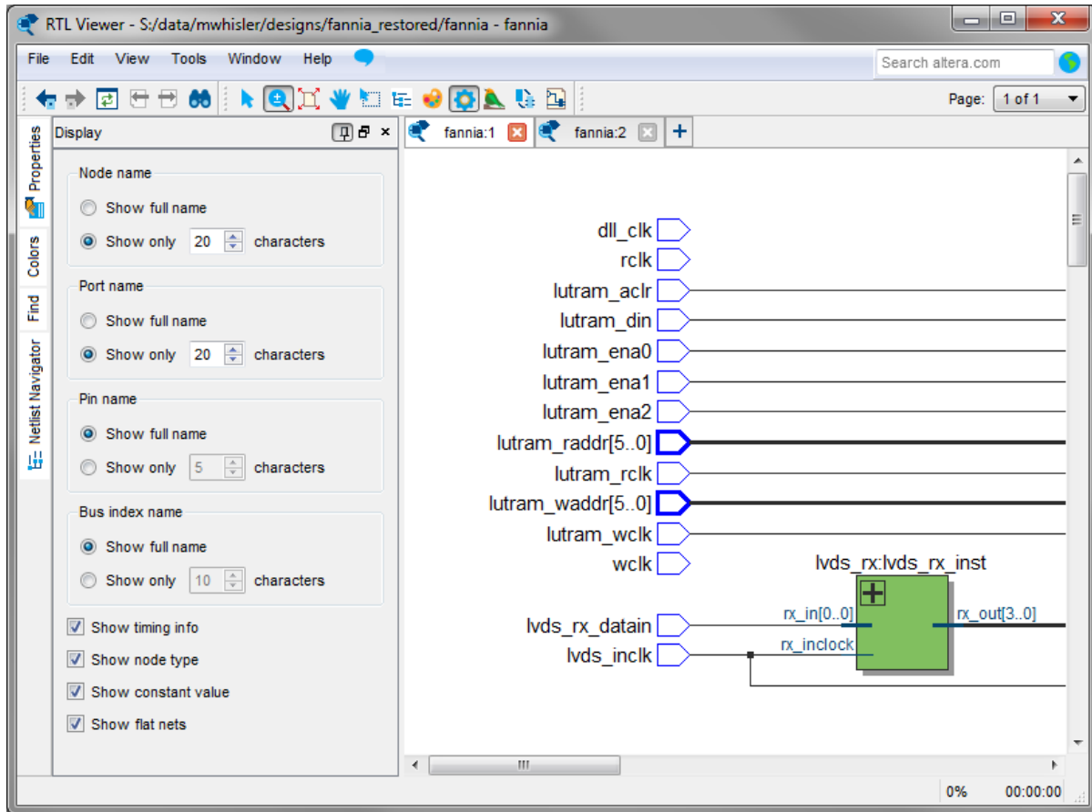
Figure 17-3: Display Settings
