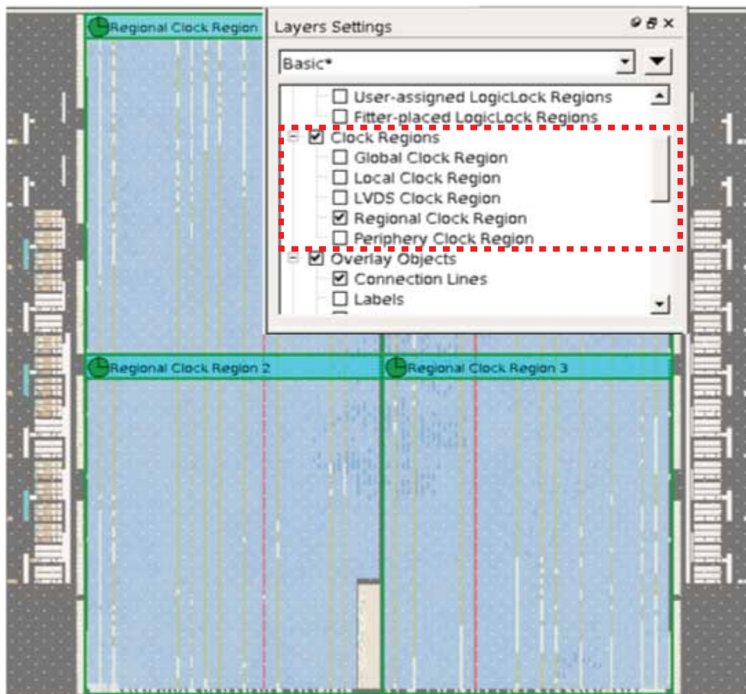
Figure 12-24: Clock Regions
