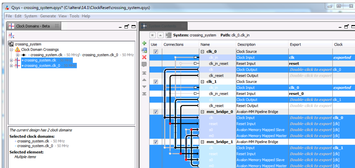
Figure 5-27: Clock Domains
