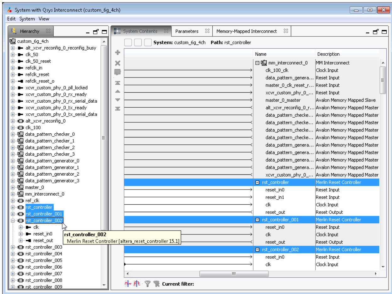
Figure 8-32: Qsys Interconnect
