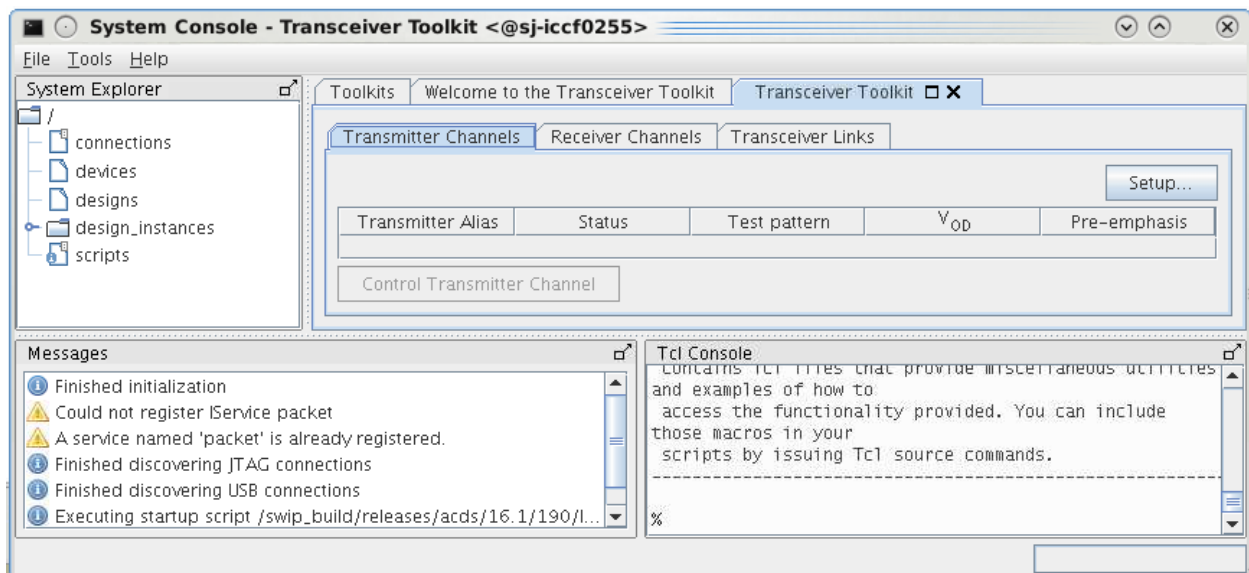
Figure 11-1: Transceiver Toolkit
