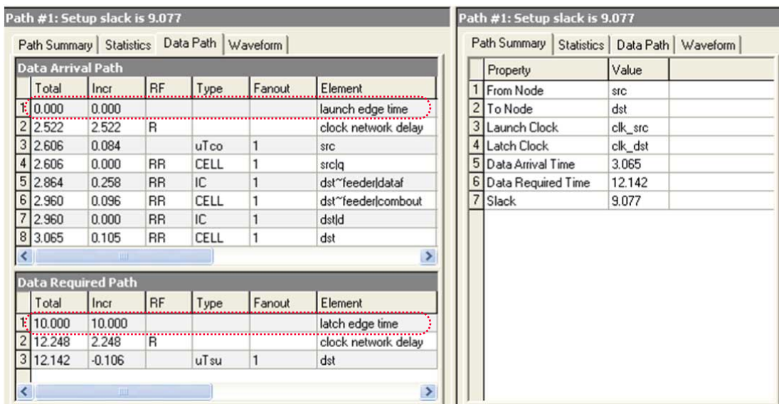
Figure 7-20: Setup Report
