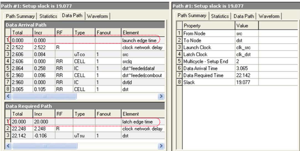
Figure 7-31: Setup Report
