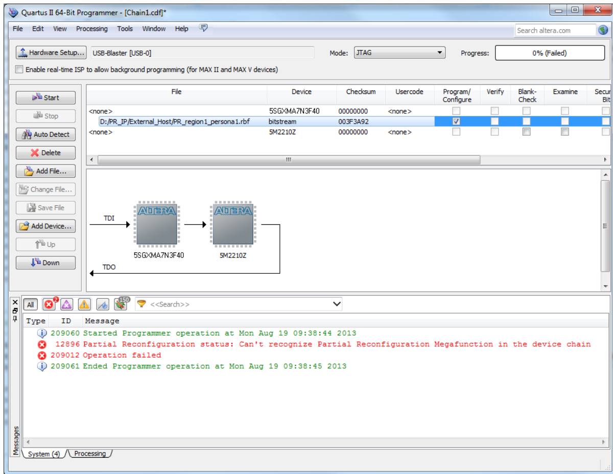
Figure 18-4: Starting PR Bitstream Configuration
