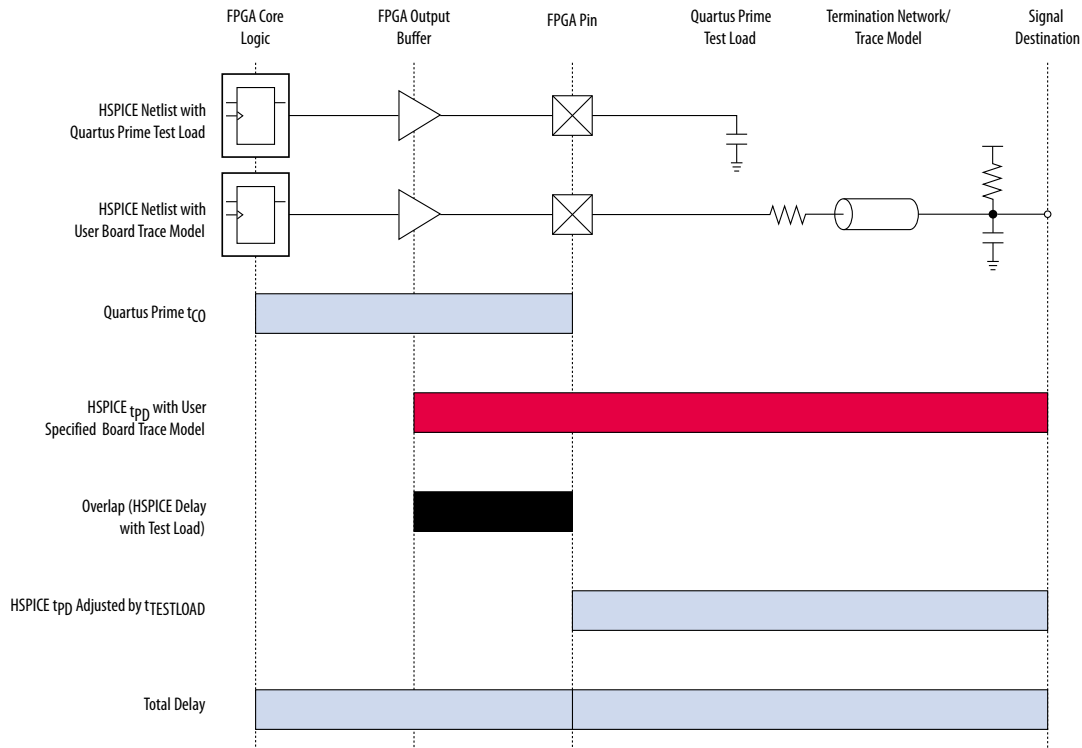
Figure 6-11: Common Test Loads Used for Output Timing
