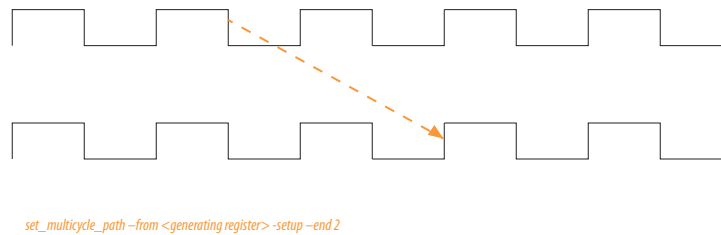
Figure 12-22: Multicycle Setup Constraint
