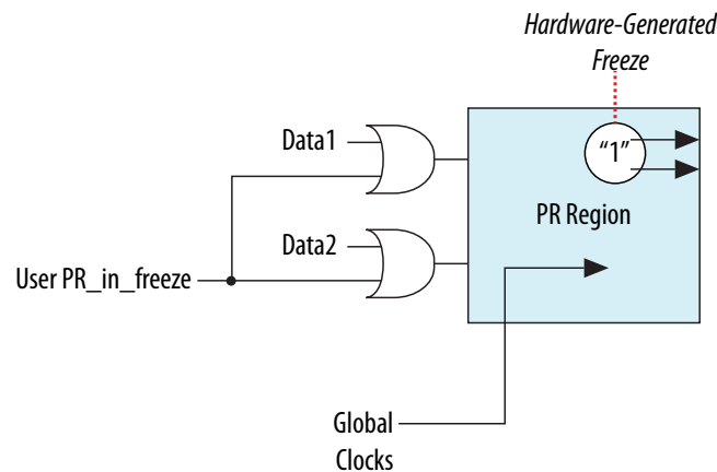
Figure 4-9: Freezing at PR Region Boundary
