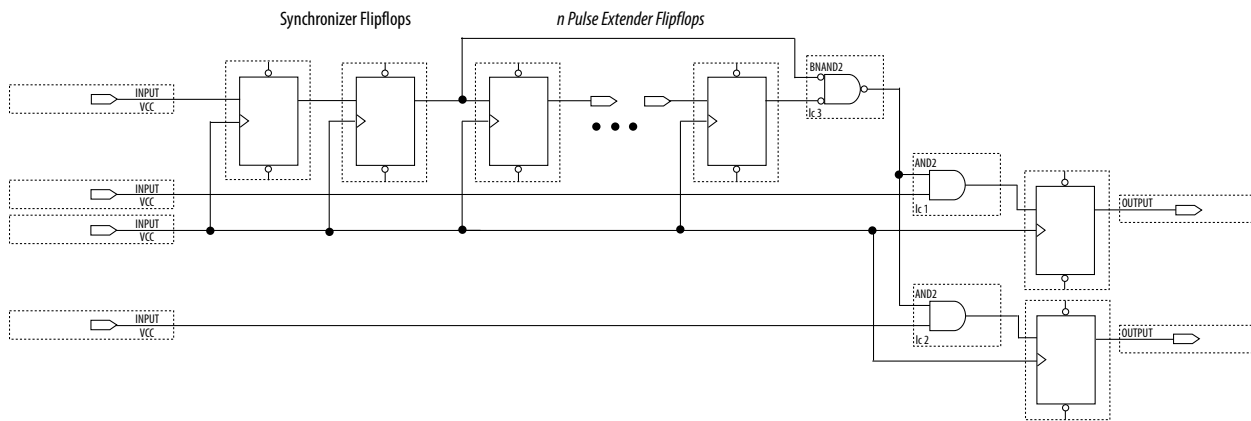
Figure 11-18: Internally Synchronized Reset with Pulse Extender
