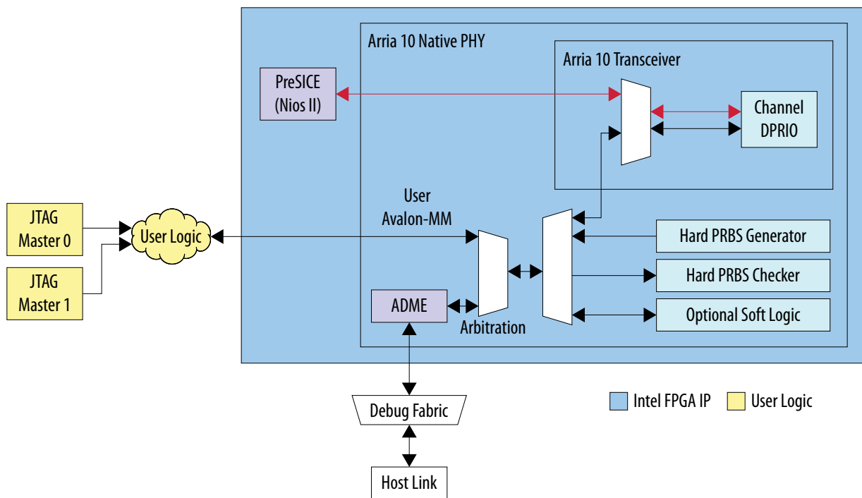
Figure 11-2: Altera Debug Master Endpoint Block Diagram
