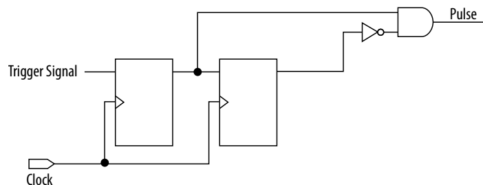
Figure 11-3: Recommended Synchronous Pulse-Generation Technique
