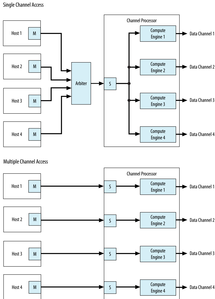
Figure 8-7: Single Interface Versus Multiple Interfaces
