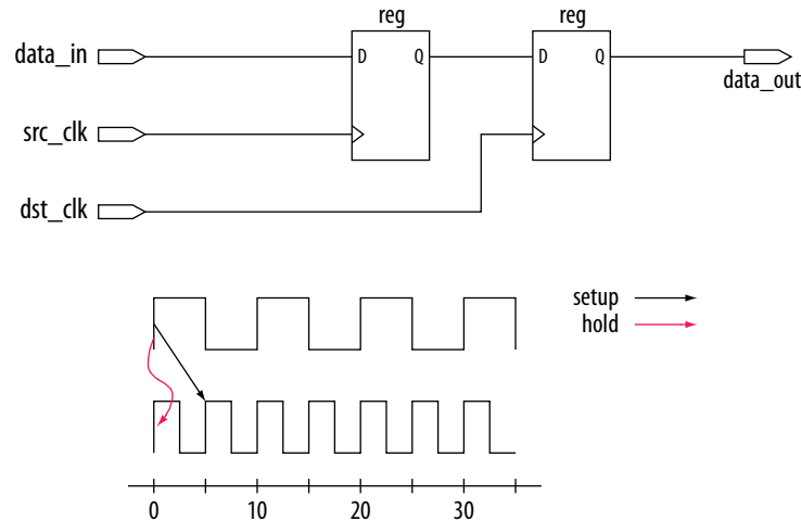
Figure 6-20: Register-to-Register Path and Default Setup and Hold Timing Diagram
