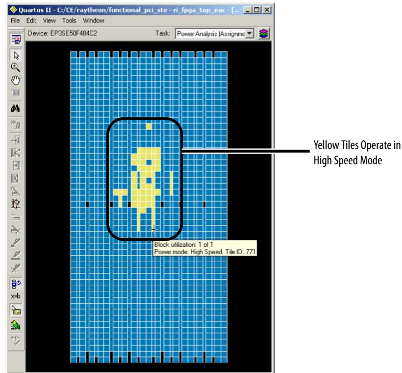
Figure 15-8: Viewing High-Speed and Low Power Tiles in a Stratix Device
