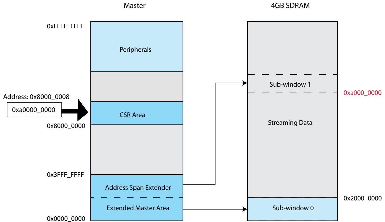
Figure 10-18: Memory mapping for Address Span Extender
