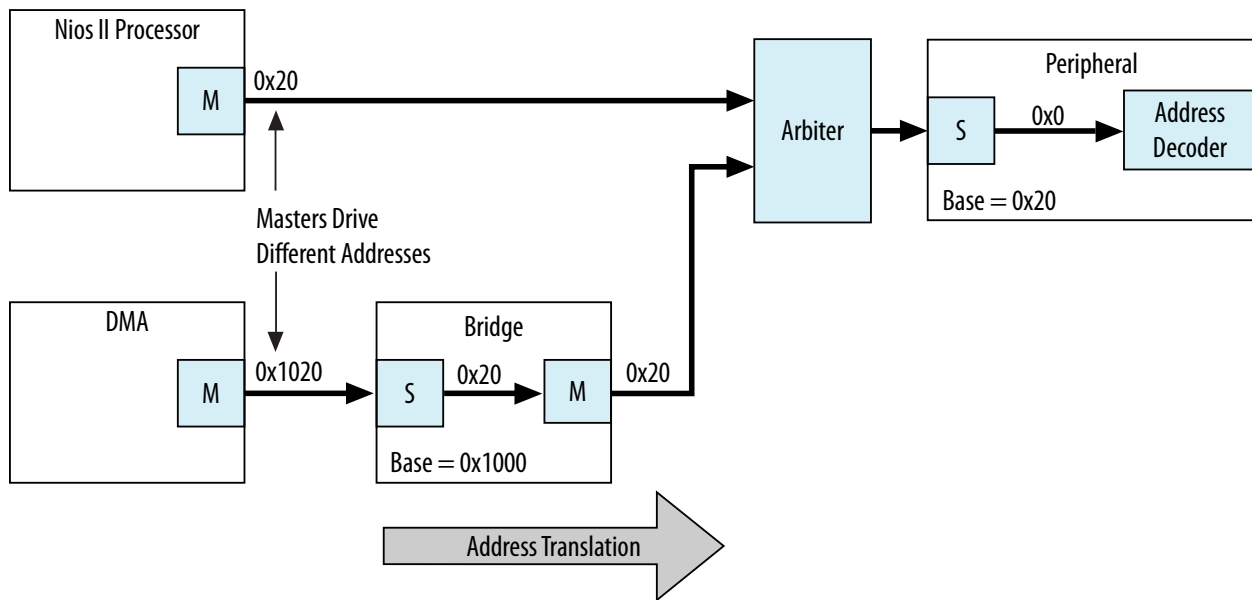
Figure 8-19: Slaves at Different Addresses and Complicating the System
