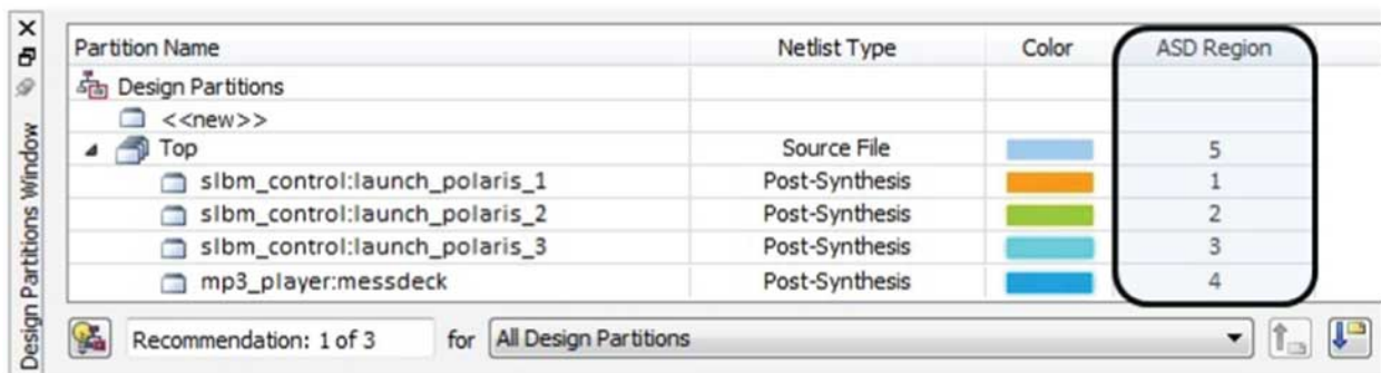
Figure 15-6: ASD Region Column in the Design Partitions Window
