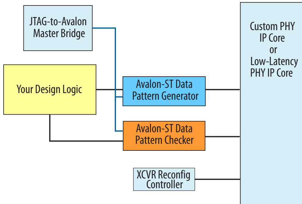
Figure 11-7: Bit Error Rate Test Configuration (Stratix V)
