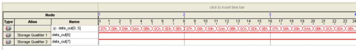
Figure 13-16: Data Acquisition of a Recurring Data Pattern in Conditional Capture Mode
