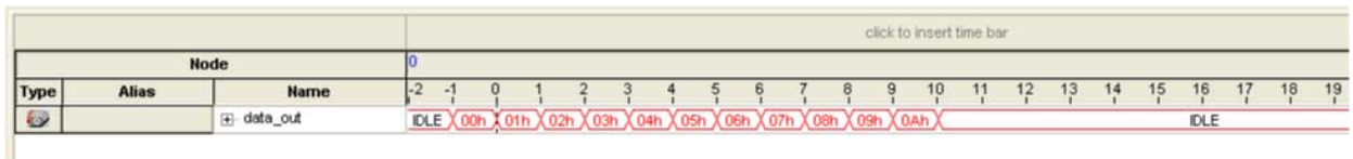
Figure 13-12: Data Acquisition of a Recurring Data Pattern in Continuous Capture Mode (Transitional Mode)
