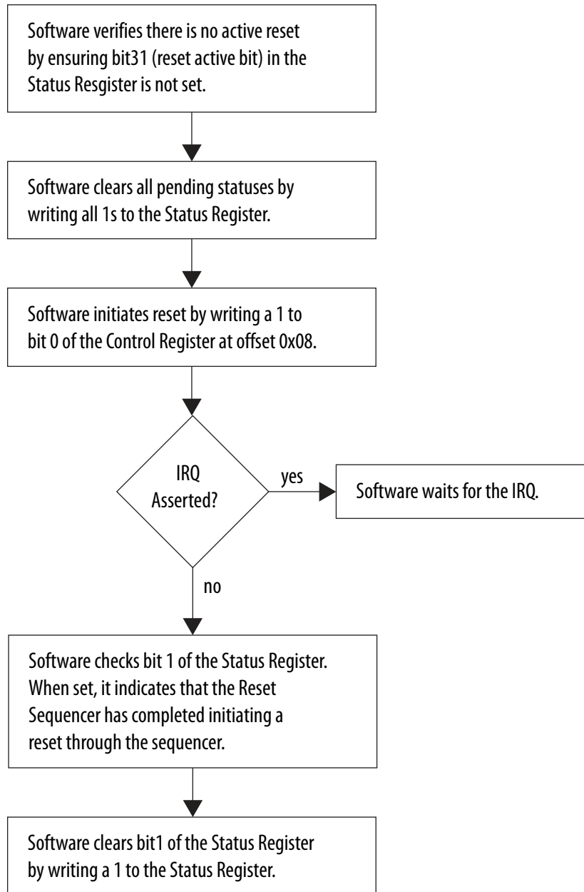
Figure 7-32: Reset Sequencer (Software-Triggered) Flow
