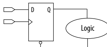
Figure 11-1: Combinational Loop Through Asynchronous Control Pin
