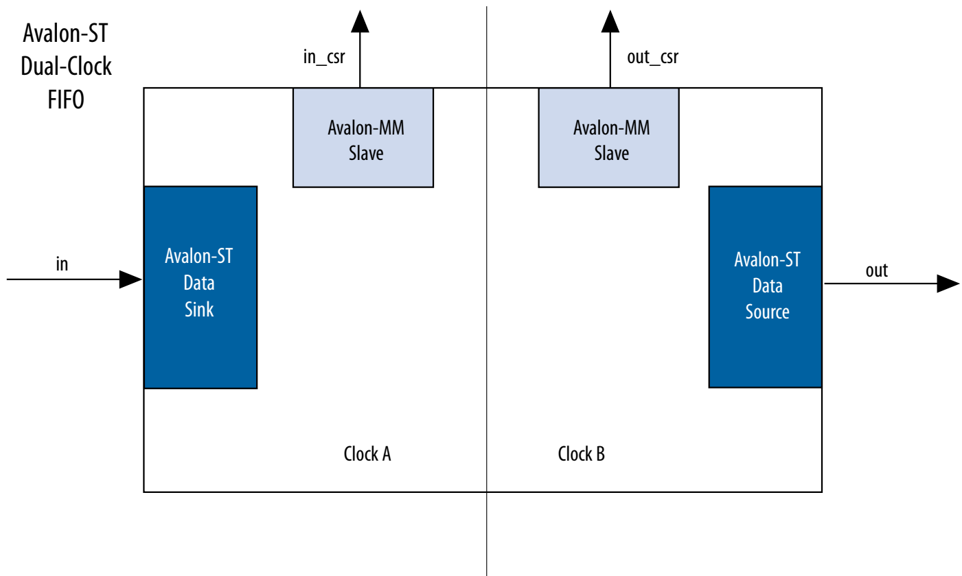
Figure 10-38: Avalon-ST Dual Clock FIFO Core
