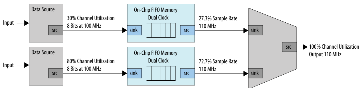
Figure 8-34: Datapath that Doubles the Clock Frequency
