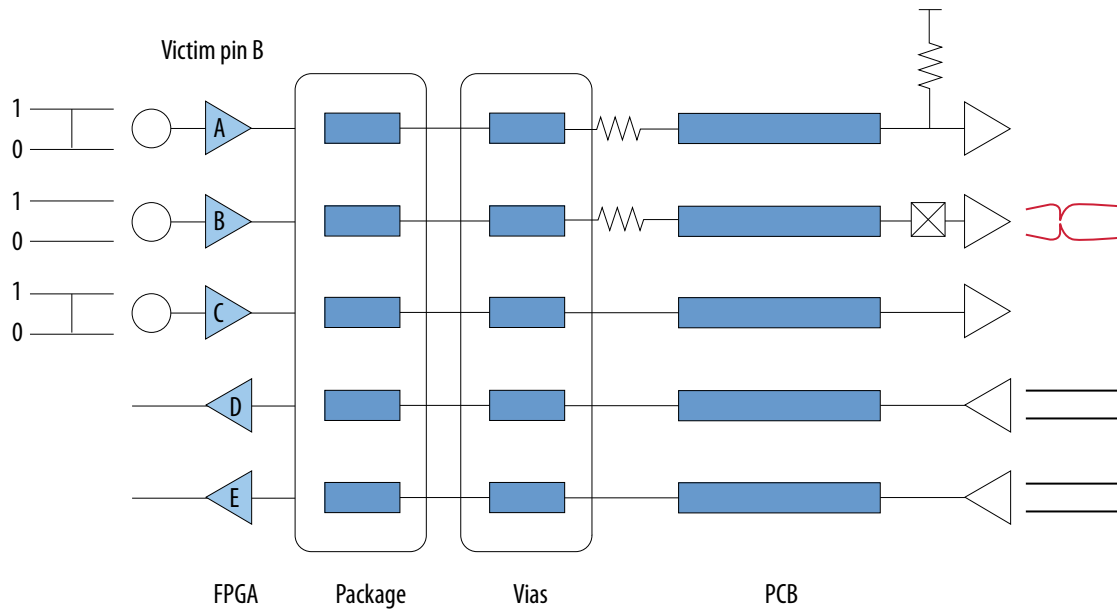
Figure 3-2: Quiet High Output Noise Estimation on Pin B
