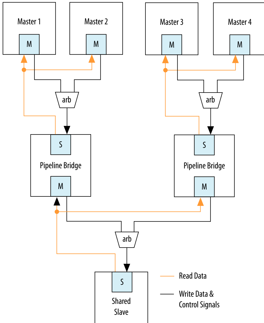
Figure 8-10: Tree of Bridges
