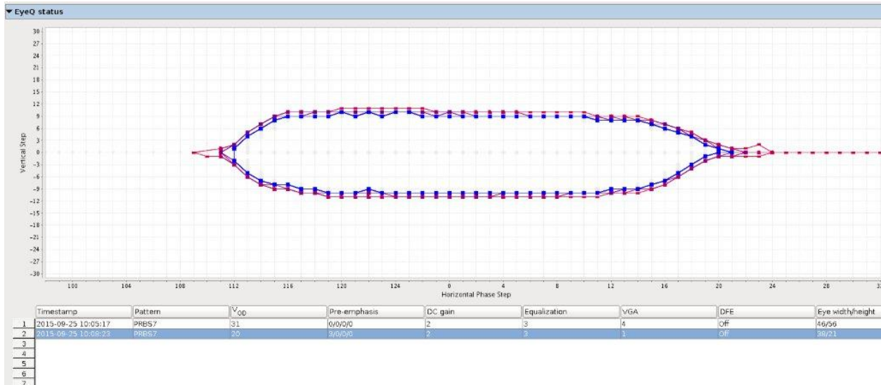
Figure 11-17: EyeQ Settings and Status Showing Results of Two Test Runs
