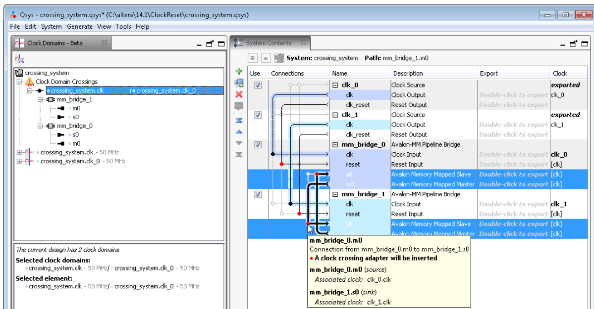
Figure 5-28: Clock Domain Crossings
