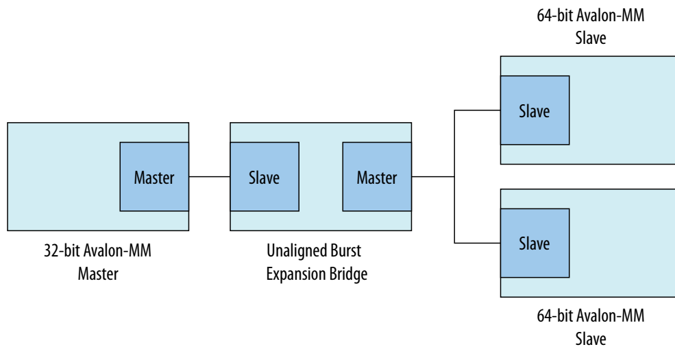
Figure 10-5: Avalon-MM Unaligned Burst Expansion Bridge
