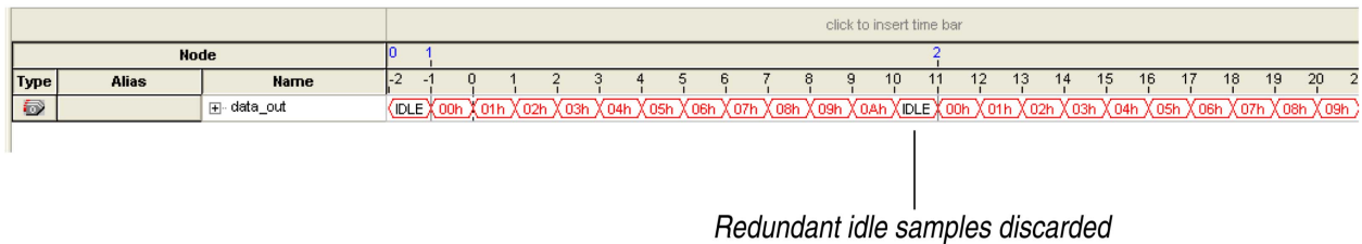
Figure 13-13: Data Acquisition of Recurring Data Pattern Using a Transitional Mode as a Storage Qualifier
