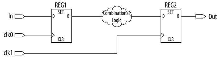
Figure 7-35: Same Frequency Clocks with Destination Clock Offset
