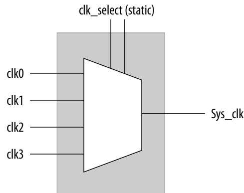
Figure 12-2: Simple Clock Multiplexer in a 6-Input LUT
