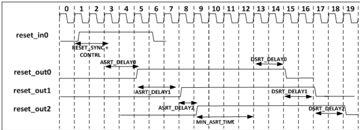
Figure 7-30: Basic Sequencing
