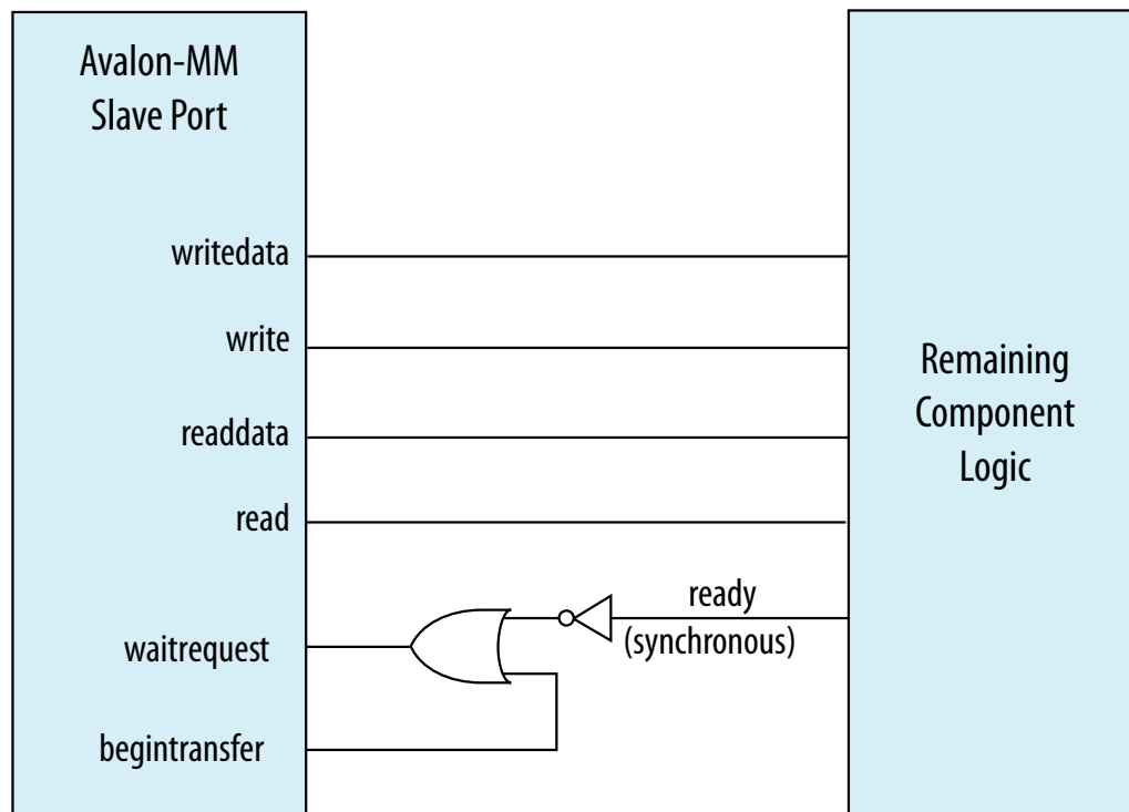
Figure 8-26: Variable Latency
