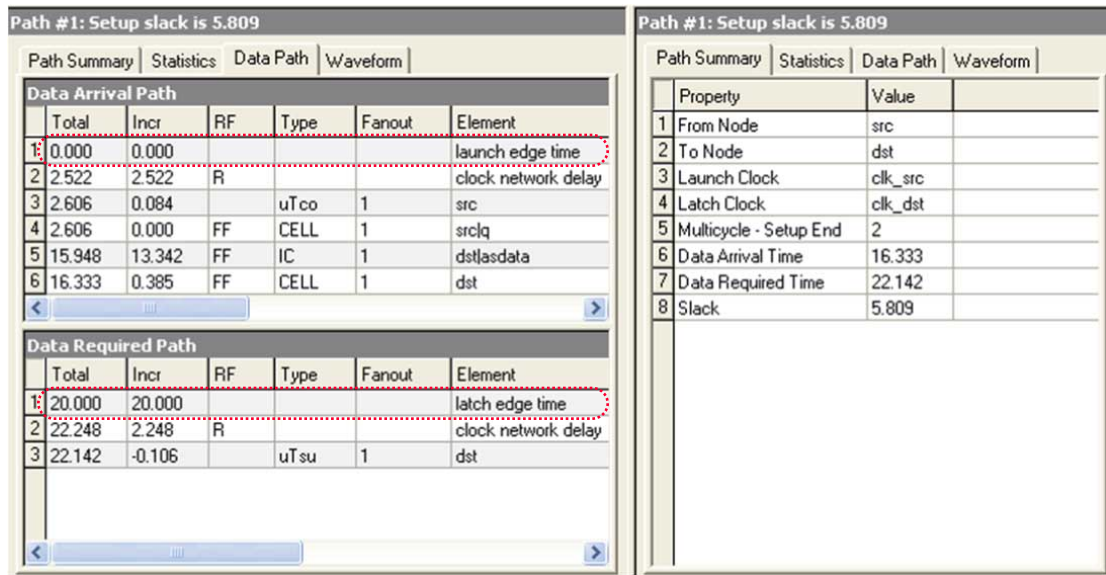
Figure 7-25: Setup Report
