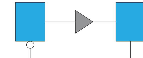
Figure 12-21: Negative-Edge Triggered Register
