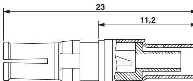
Dimensioned drawing
