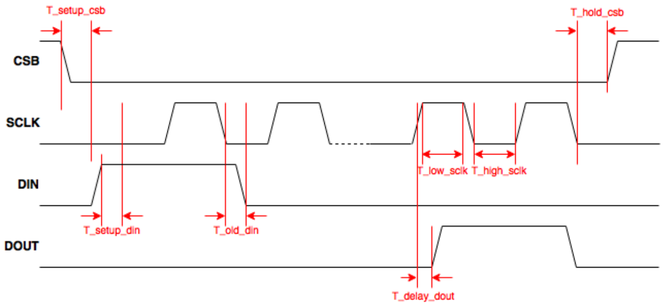
Figure 15 : SPI timing diagram
