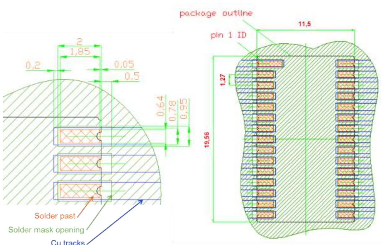
Figure 7: PCB Footprint
