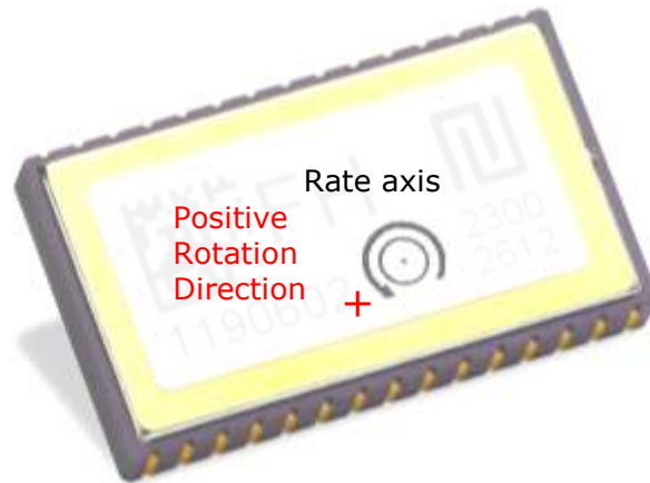
Figure 2: Axial orientation (Top side facing up with marking)
