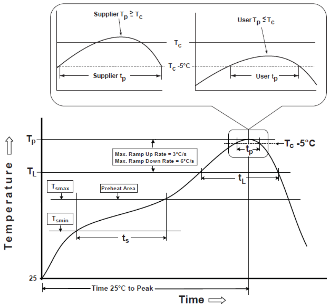
Figure 6: Recommended reflow profile (JEDEC)
