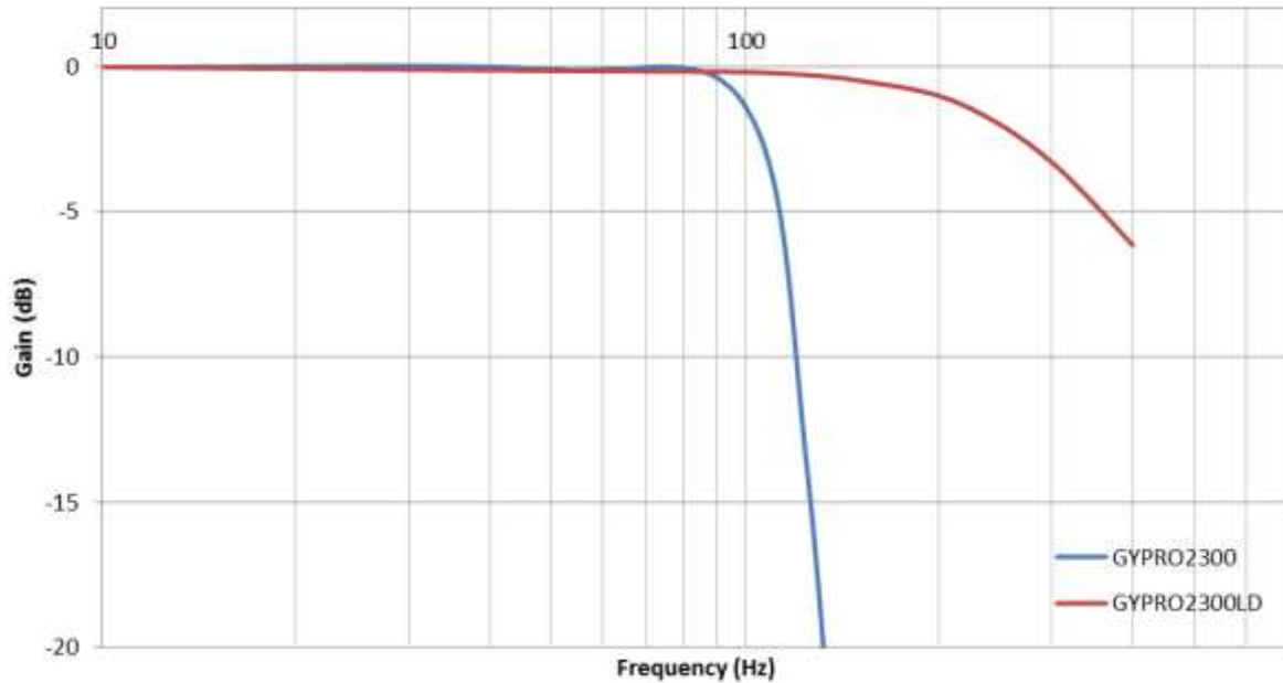
Figure 13: GYPRO2300 and GYPRO2300LD frequency response
