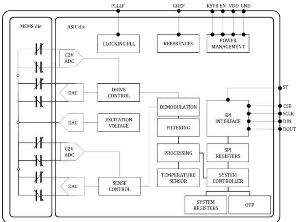
Figure 1: GYPRO2300 sensor block diagram
