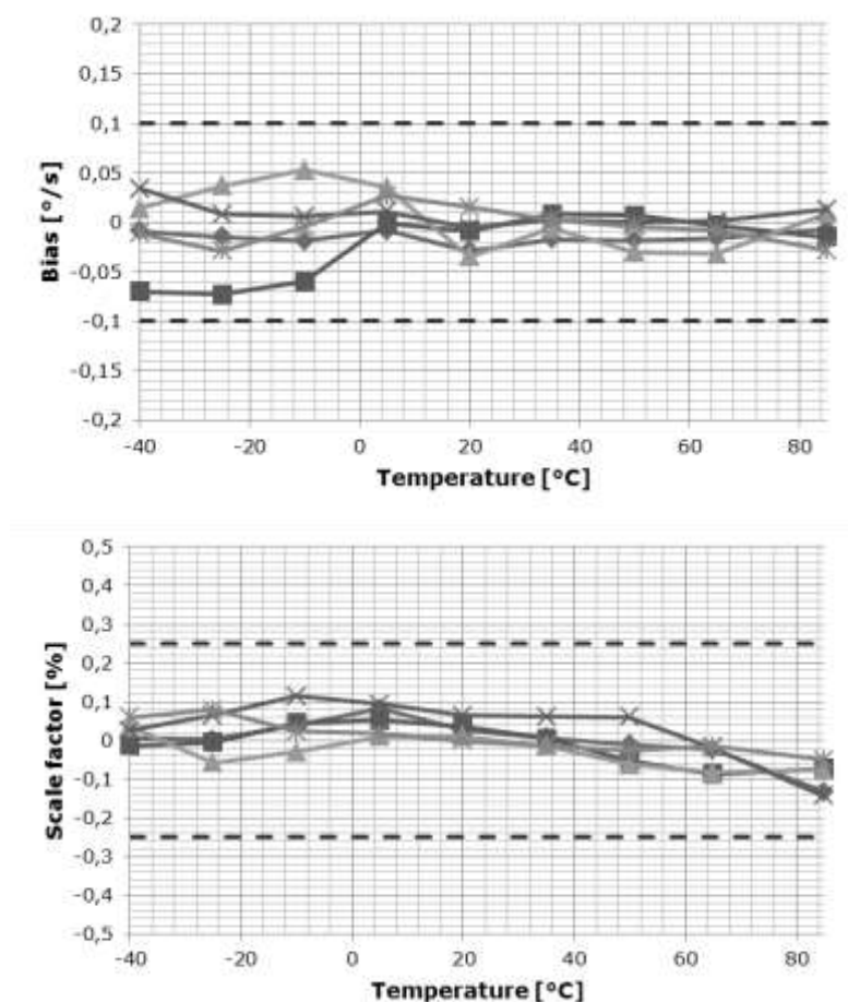
Figure 10: Temperature-compensated Bias and Scale Factor versus temperature Dotted lines correspond to the max specifications
