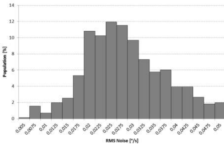
Figure 11: GYPRO2300 RMS noise distribution on 500 sensors
