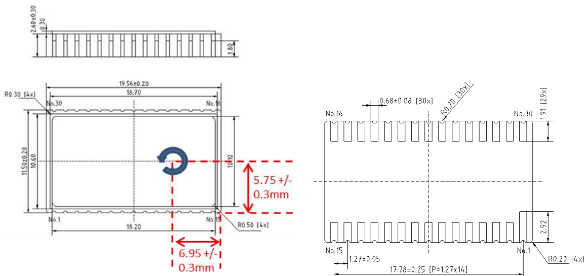
Figure 3: Outline dimensions including the package lid (shown in millimeters). Proof mass center is located at the center of the circular arrow
