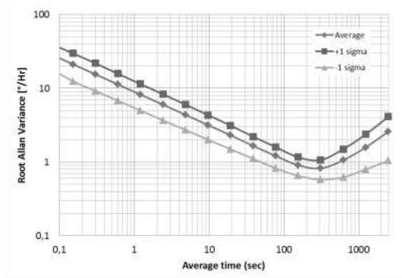
Figure 9: Root Allan variance at room temperature
