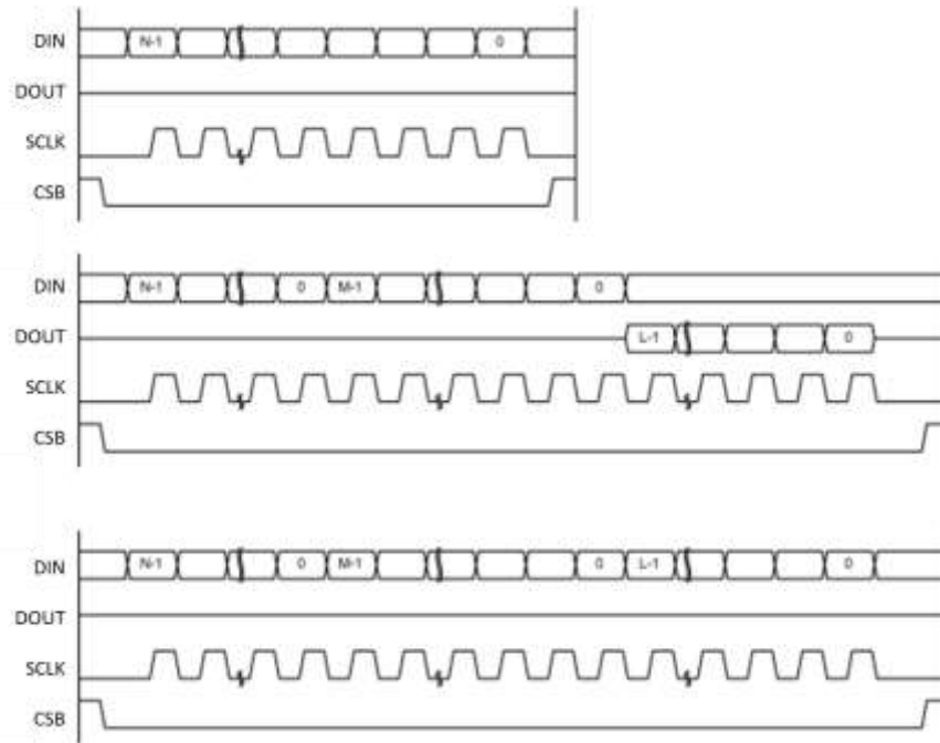
Figure 14: Different scenarios for SPI communication
