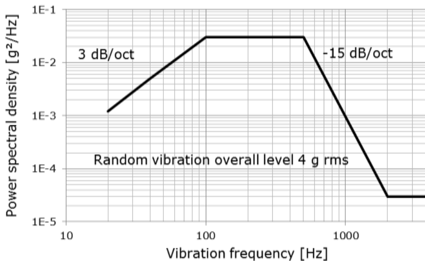
Figure 8: Random vibration profile for bias rectification
