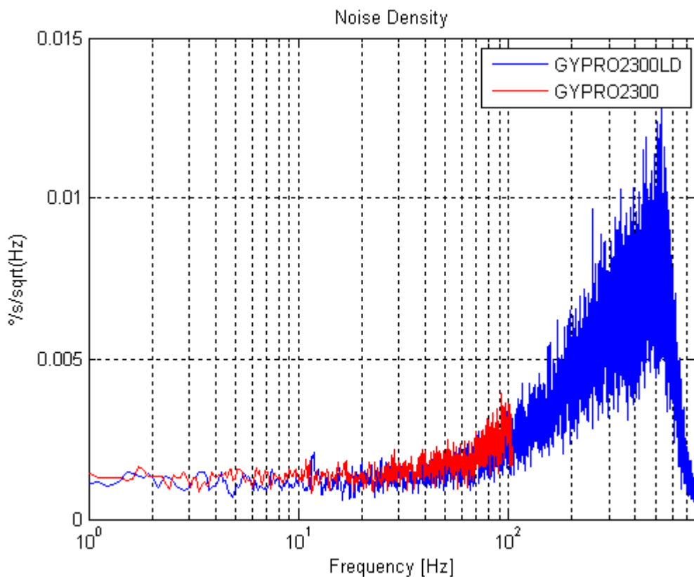
Figure 12: Noise density for GYPRO2300 and GYPRO2300LD (typical)
