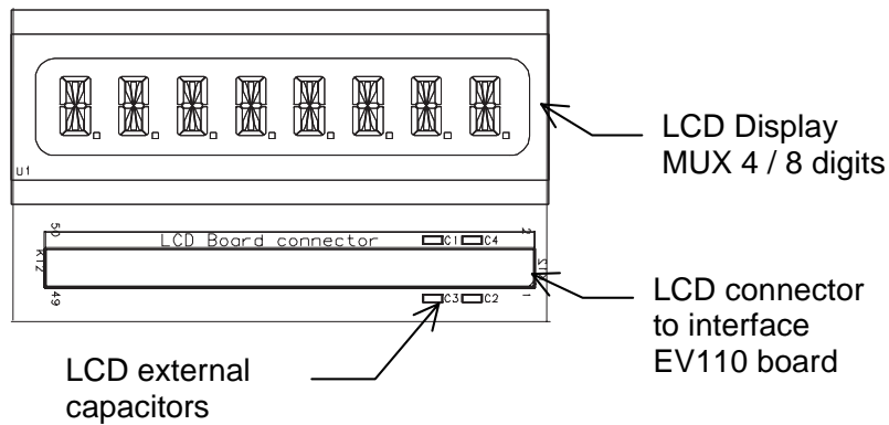
Figure 4 LCD board hardware layout
