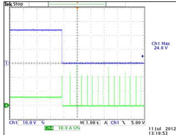
24V OUT, 264VAC
