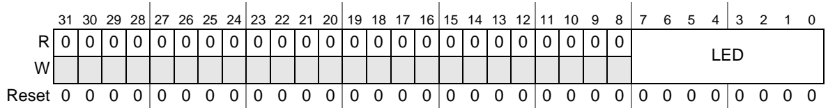
Figure 17. FPGA_7SEGMENT Register
